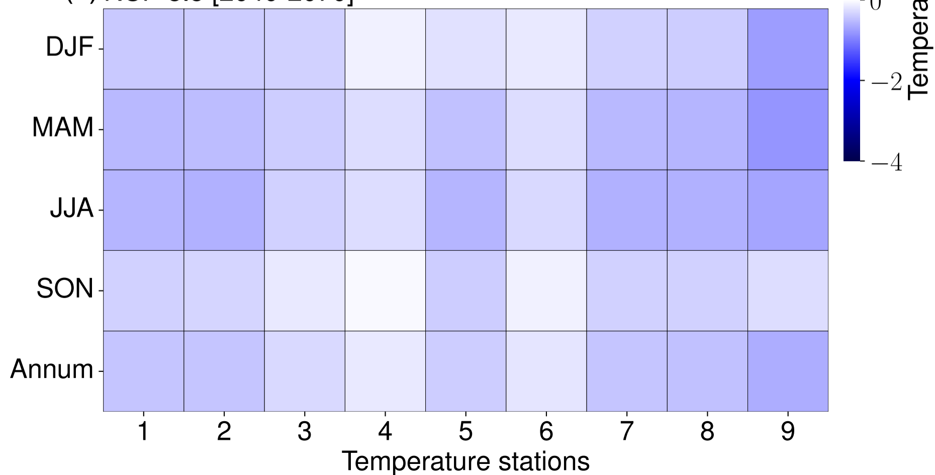
(c) RCP 8.5 [2040-2070]
