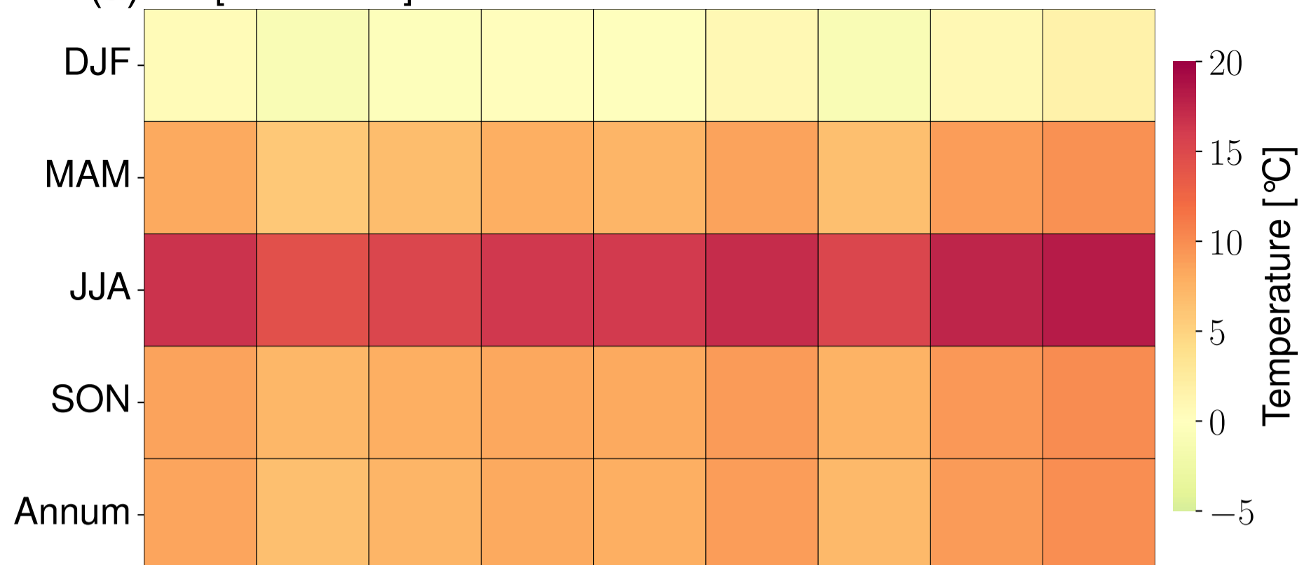
(b) RCP 2.6 [2040-2070]
