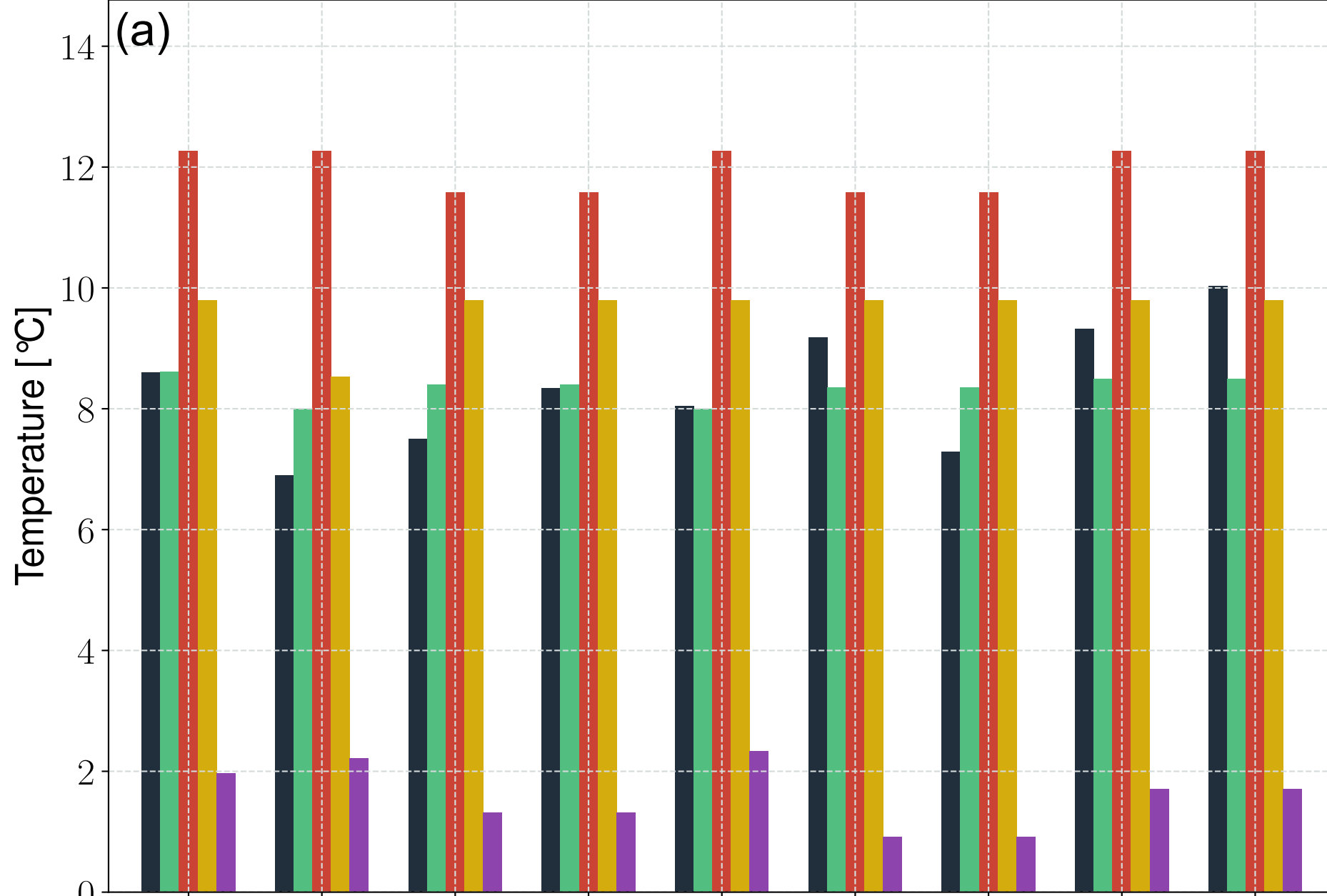
RCP 8.5 [2040-2060]
