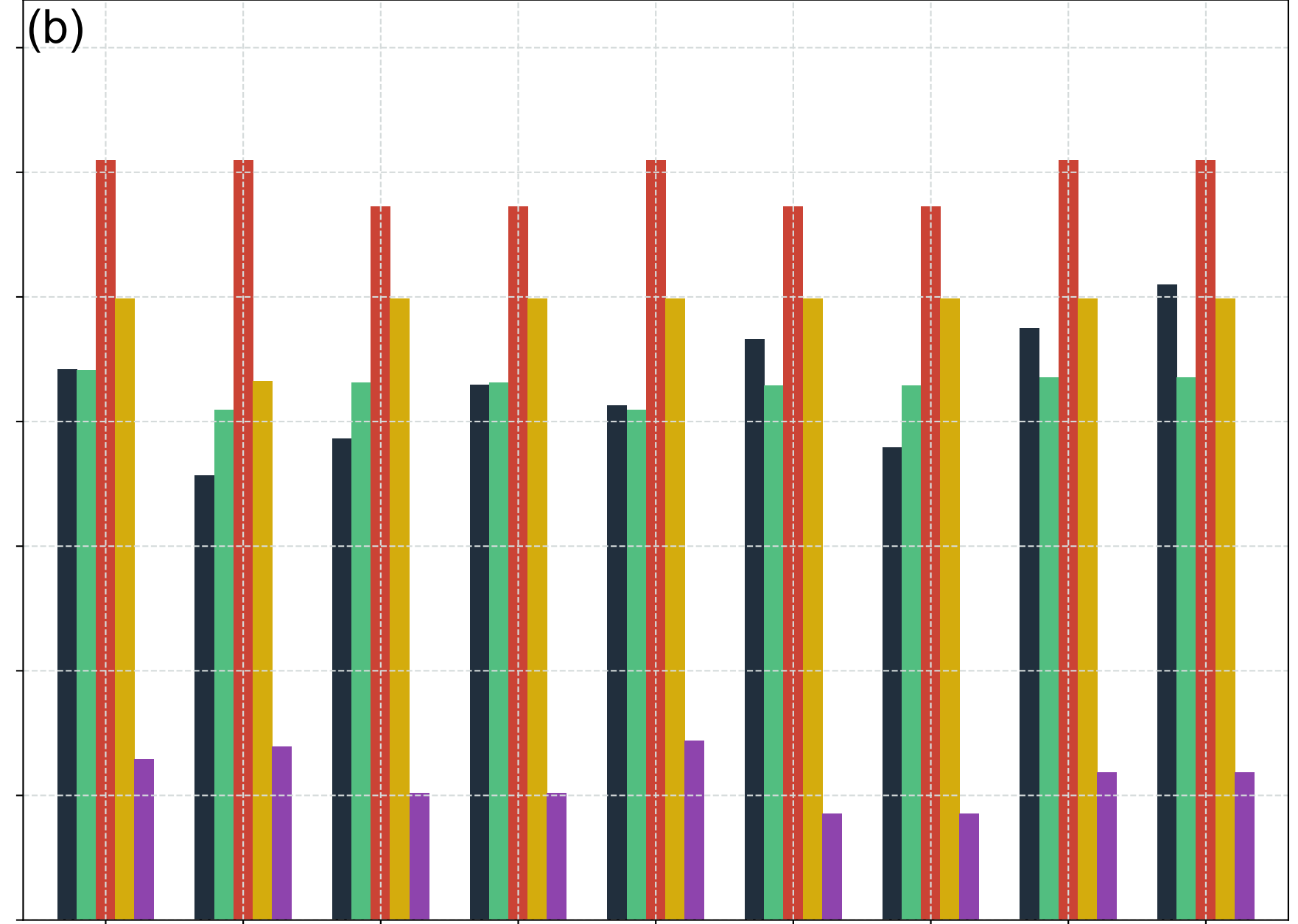
RCP 8.5 [2080-2100]
