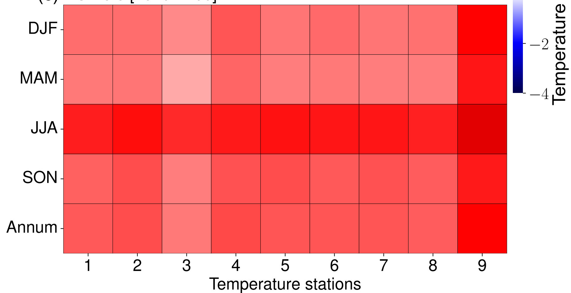
(c) RCP 8.5 [2070-2100]
