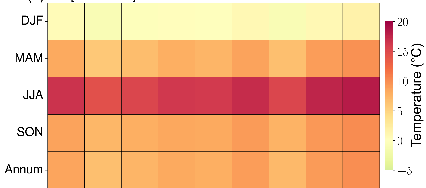
(b) RCP 2.6 [2070-2100]
