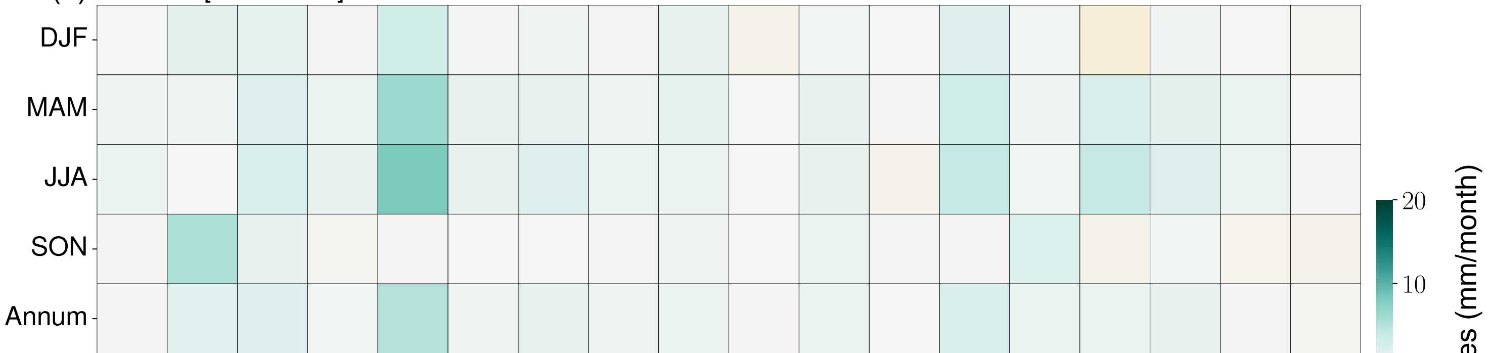
(b) RCP 2.6 [2070-2100]
