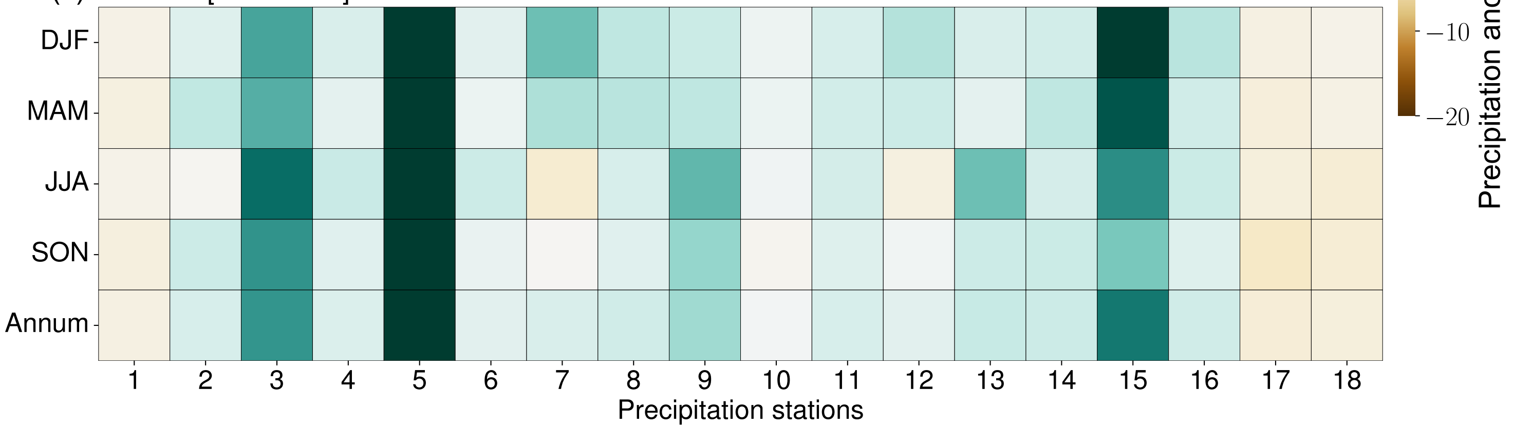
(c) RCP 8.5 [2070-2100]
