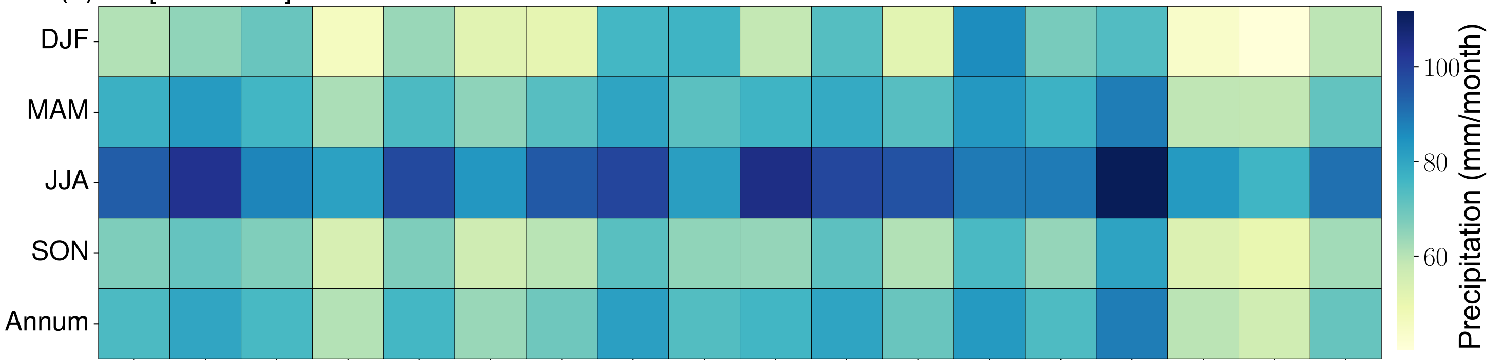
(a) obs [1958-2010]
