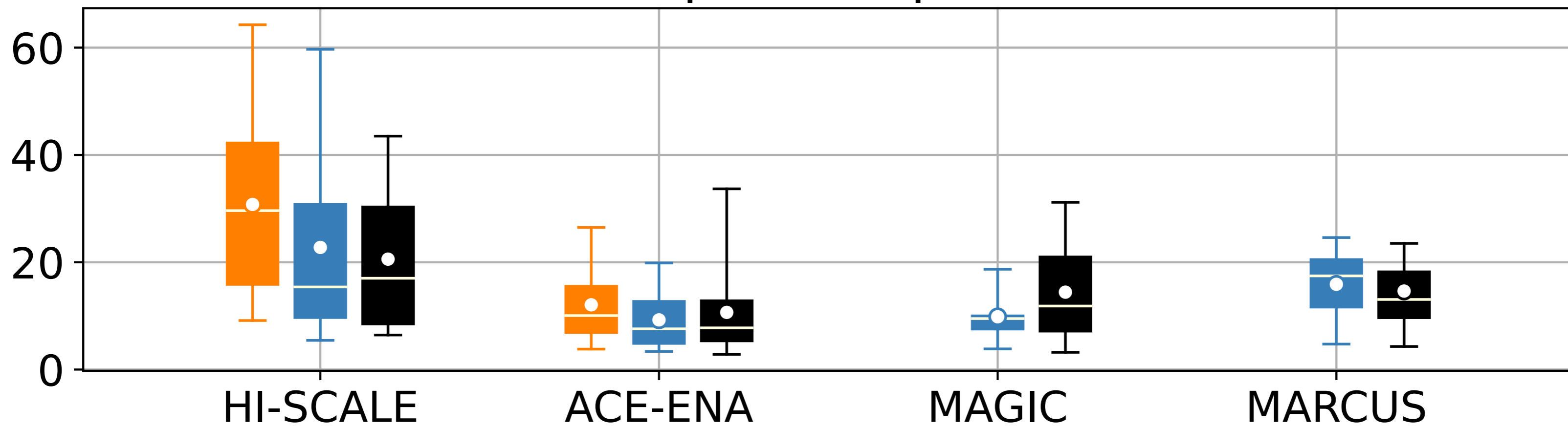
(f) Cloud Optical Depth (unitless)
