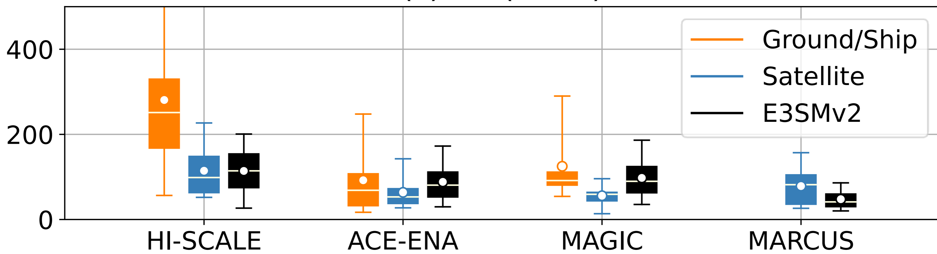
(c) Nd (cm -3 )
