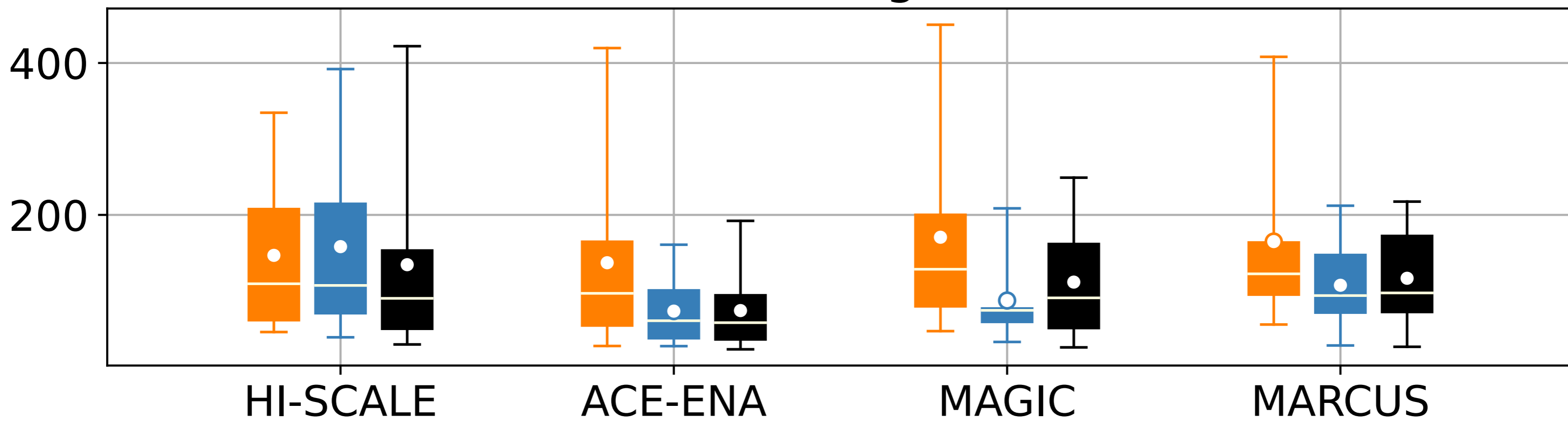
(e) Reff (μm)
