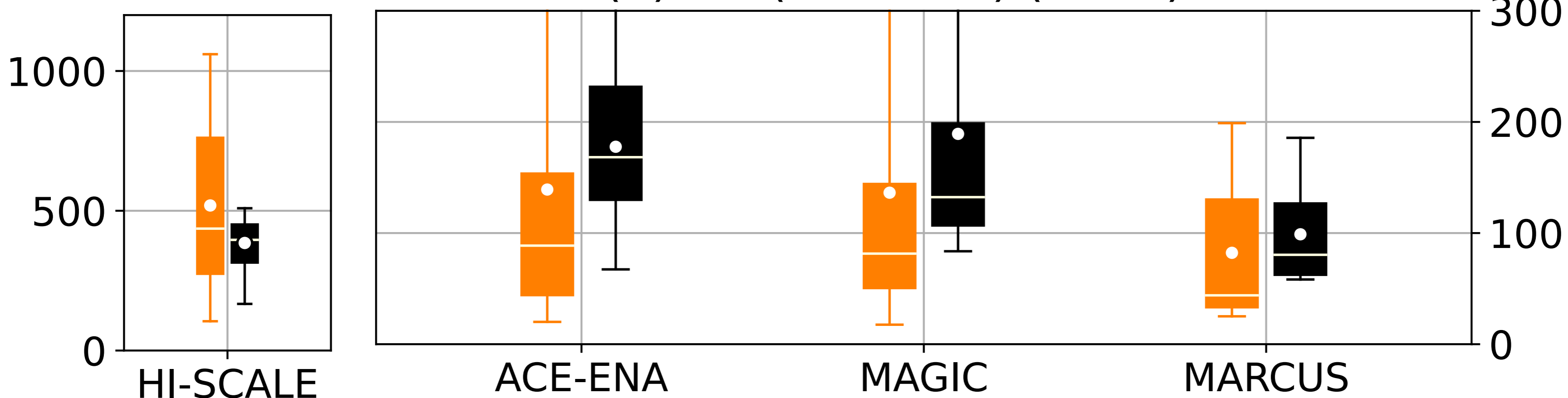
(b) CN (>100nm) (cm -3 )
