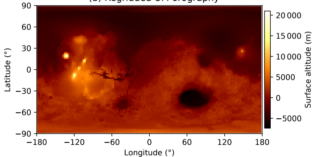
(b) Regridded UM orography
