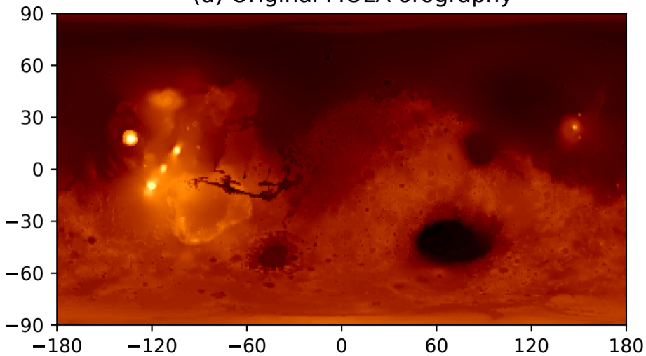
(a) Original MOLA orography
