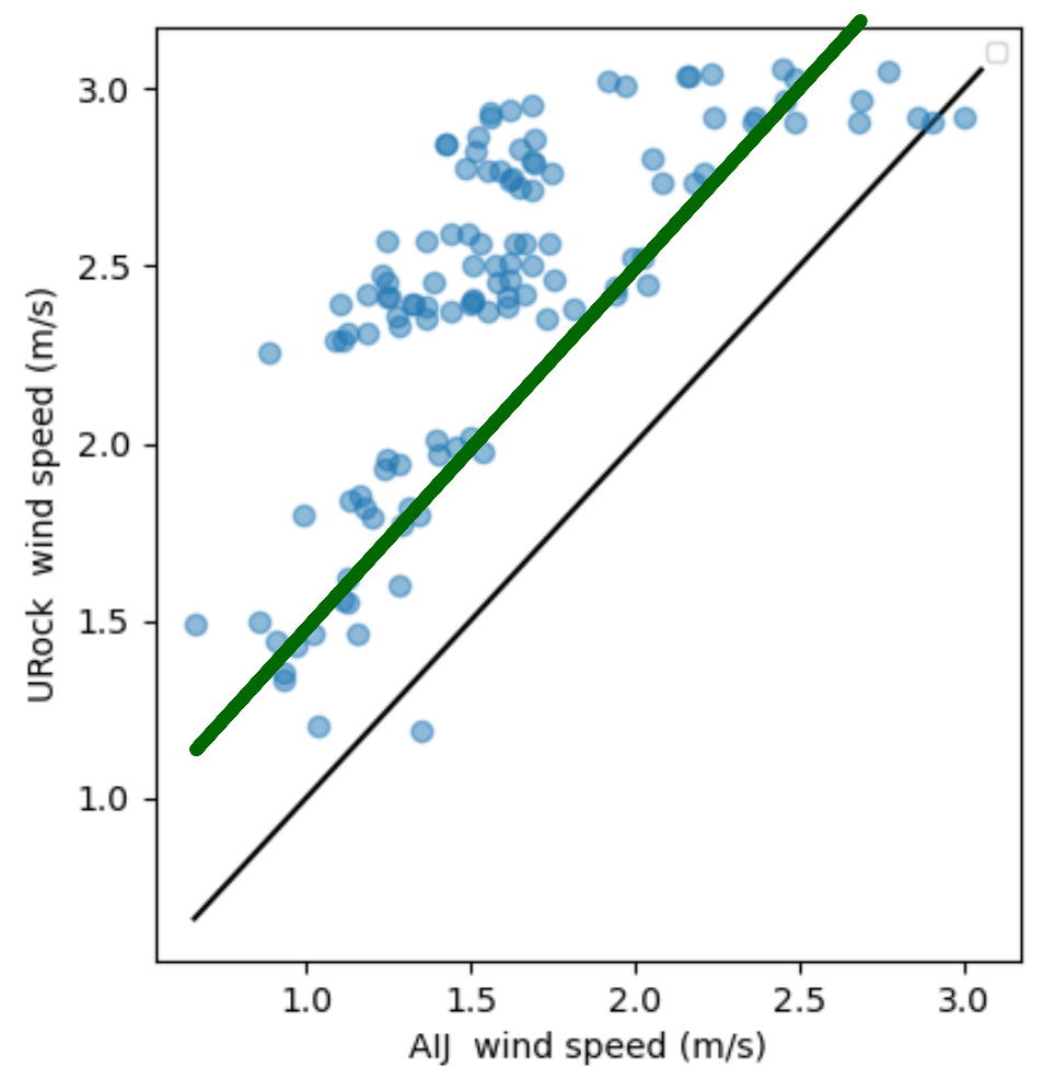
(b) Wind speed at z = 0.125 b when wind comes from West
