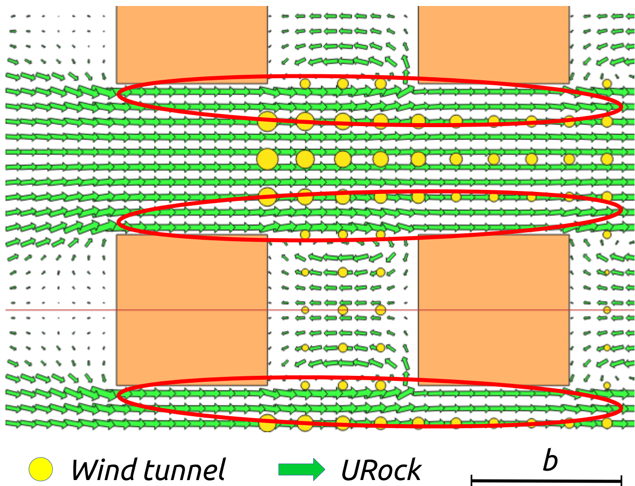
(a) Horizontal section at z = 0.125 b Wind vectors when wind comes from West
