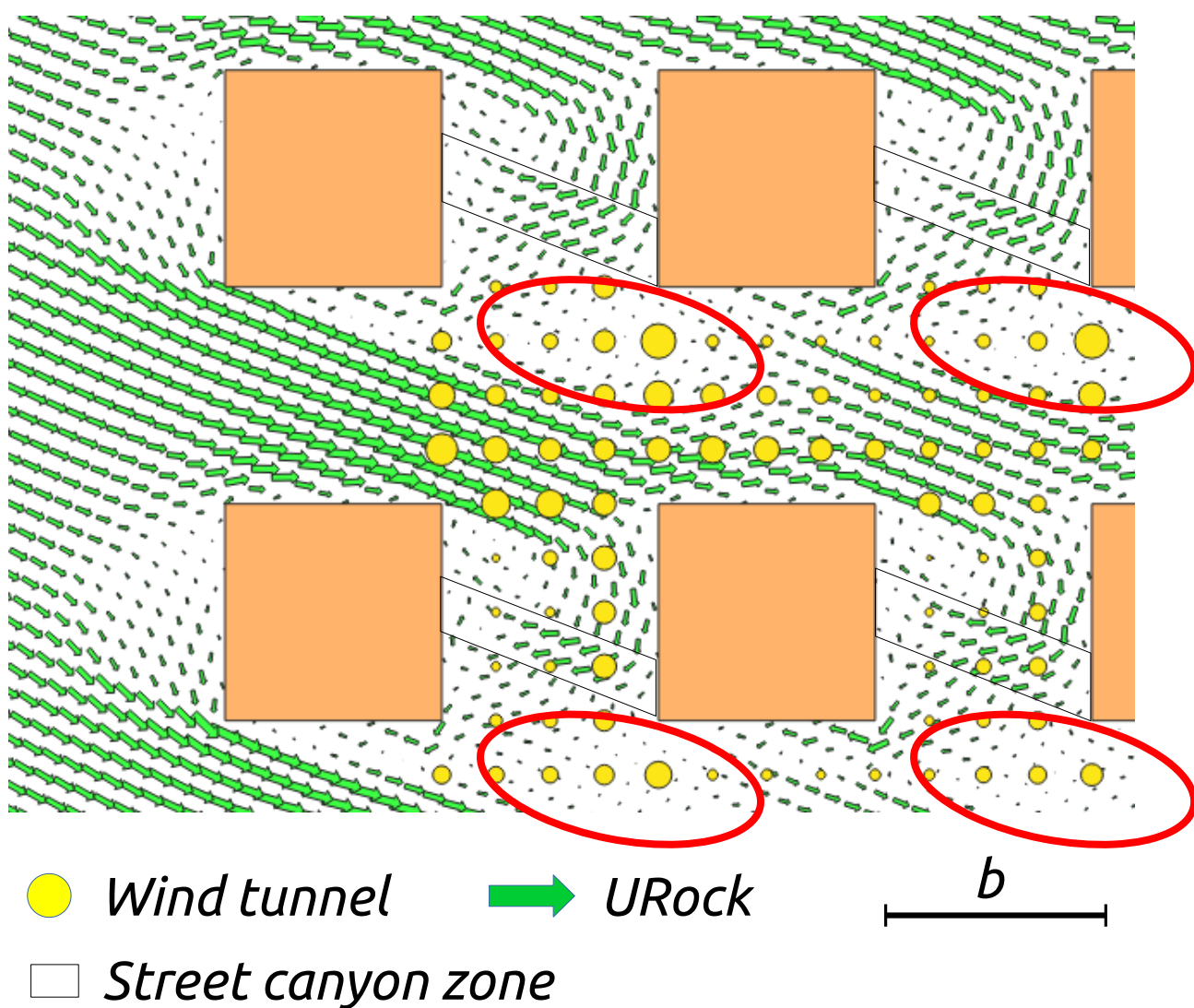
(c) Horizontal section at z = 0.125 b Wind vectors when wind comes 22° clockwise from West
