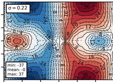
(e) Eastward Wind [ \text{m s}^{-1} ]
