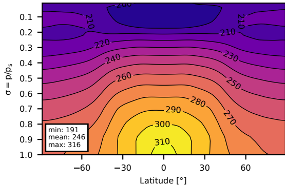
(a) Air Temperature [K]
