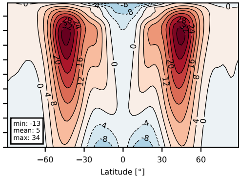
(b) Eastward Wind [ \text{m s}^{-1} ]
