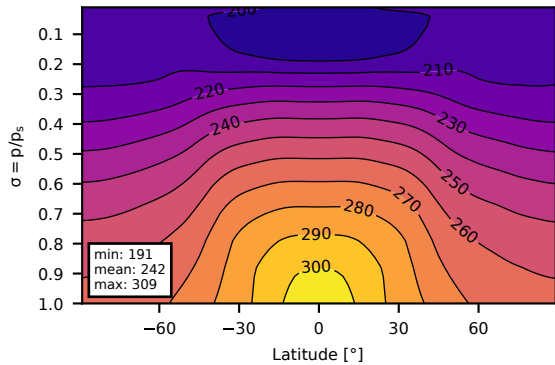
(a) Air Temperature [K]
