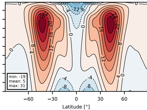
(b) Eastward Wind [ \text{m s}^{-1} ]
