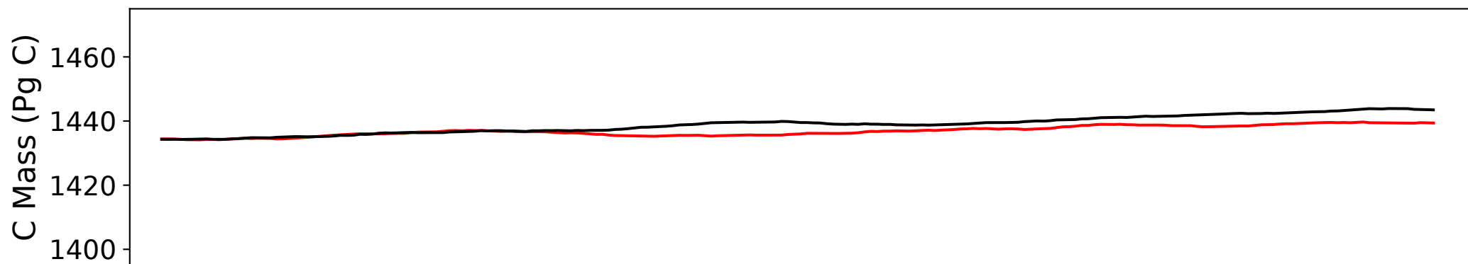
Soil carbon mass
