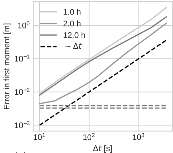
Convergence with \Delta t , Lagrangian
