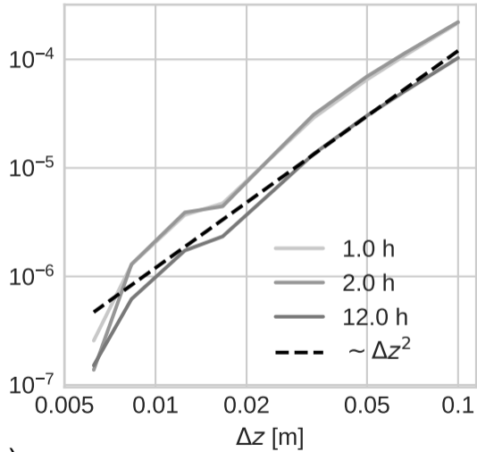
Convergence with \Delta z , Eulerian
