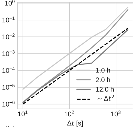
Convergence with \Delta t , Eulerian
