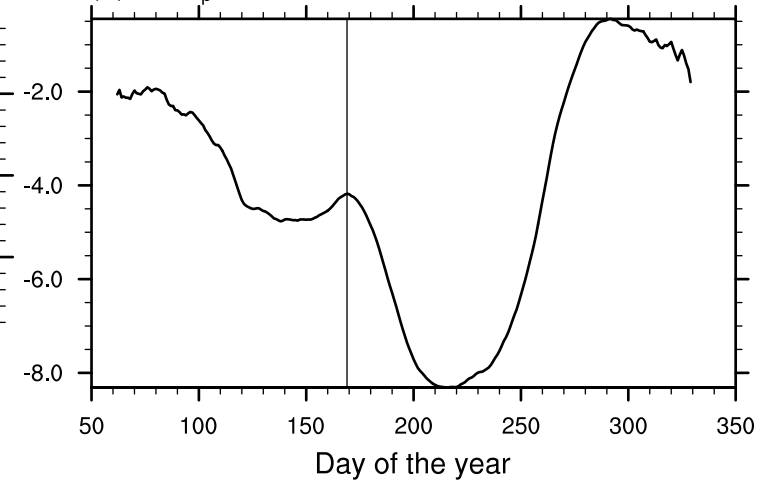
(f) \text{dex}_p
