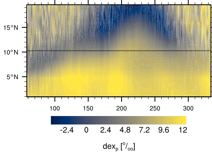
(c) \text{dex}_p
