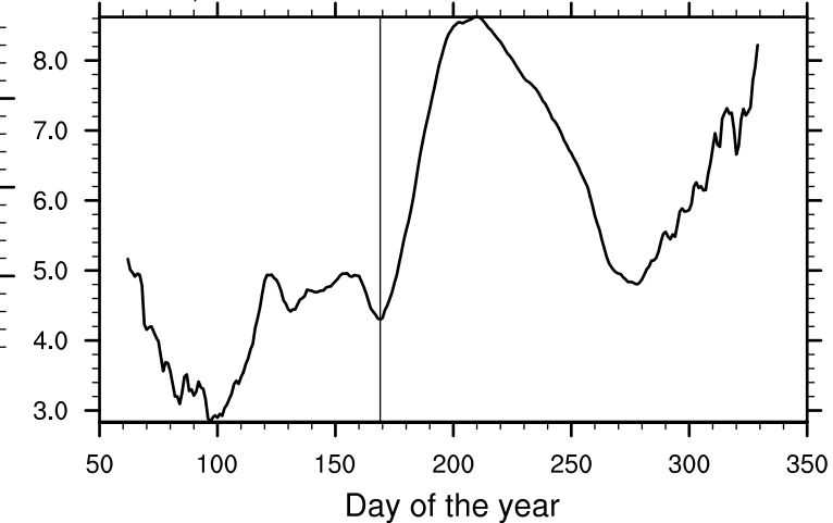
(f) \text{dex}_p
