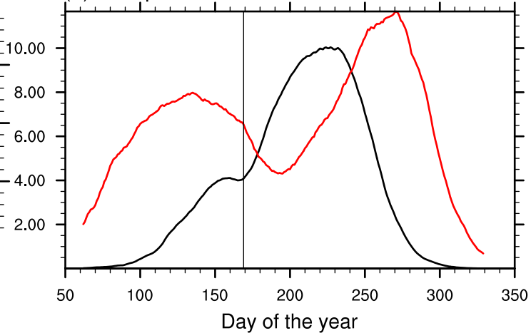
(e) \delta^{18}\text{O}_p
