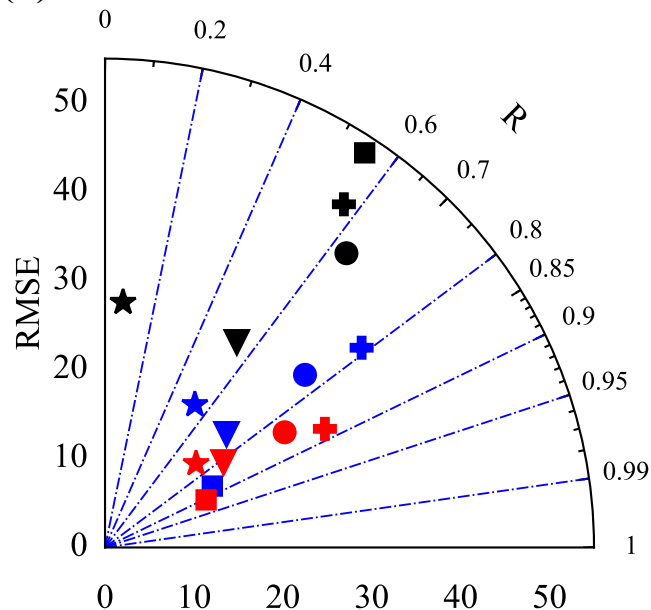
(b) Forecast 12 h in advance
