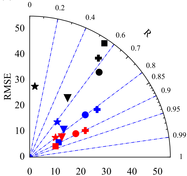
(a) Forecast 6 h in advance
