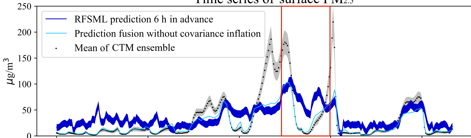
Time series of surface PM 2.5
