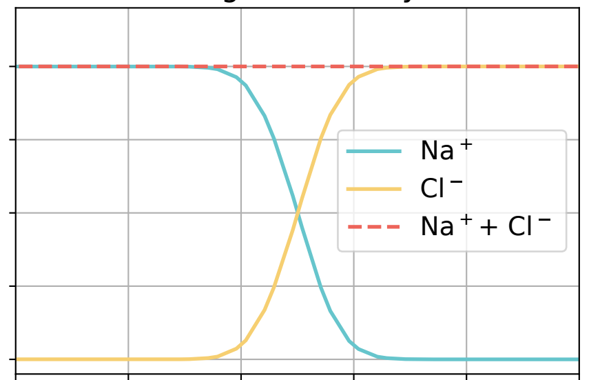
Single diffusivity
