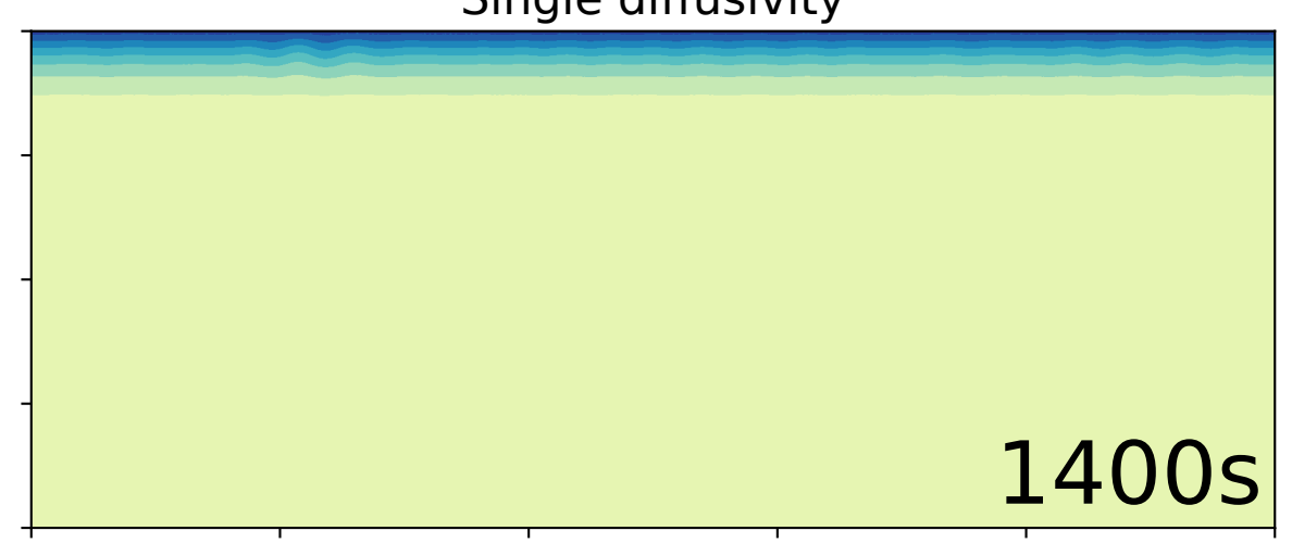
Single diffusivity
