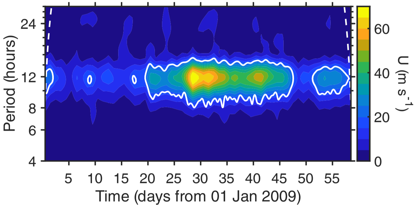
(c) Migrating semidiurnal tide at 110 km
