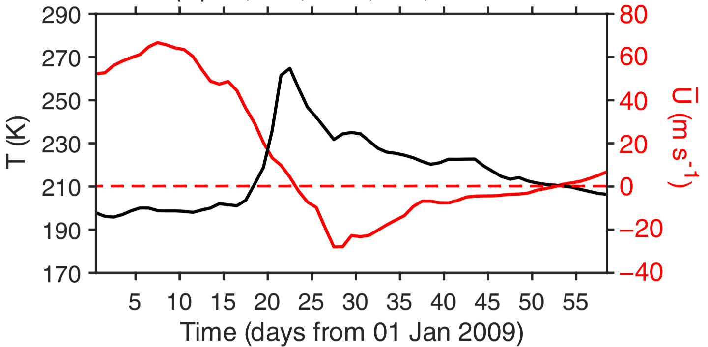
(b) Fourier-wavelet ( W2 , 50^\circ\text{N} , 110 km)
