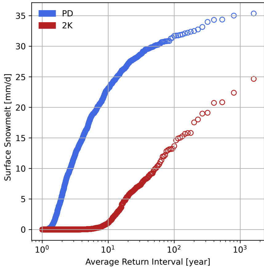
(a) Southeast Greenland July snowmelt
