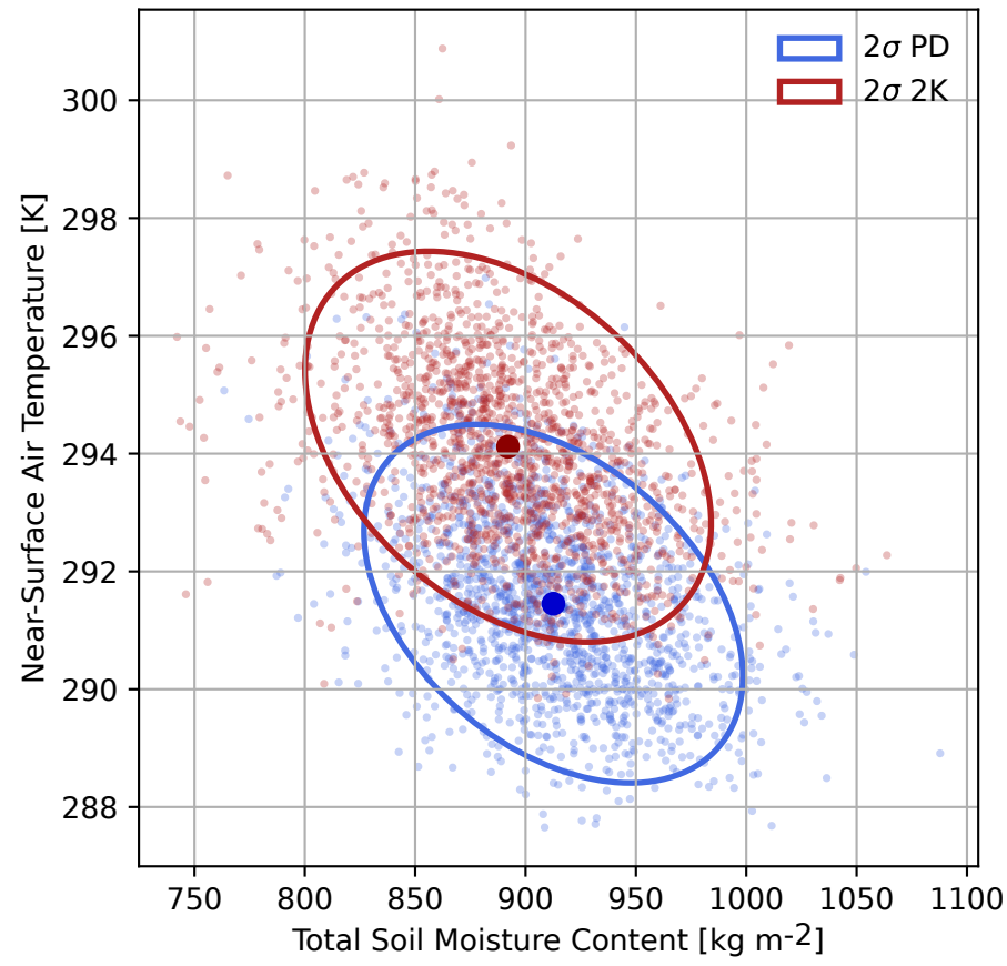
(b) Southern England July T2m/soil moisture
