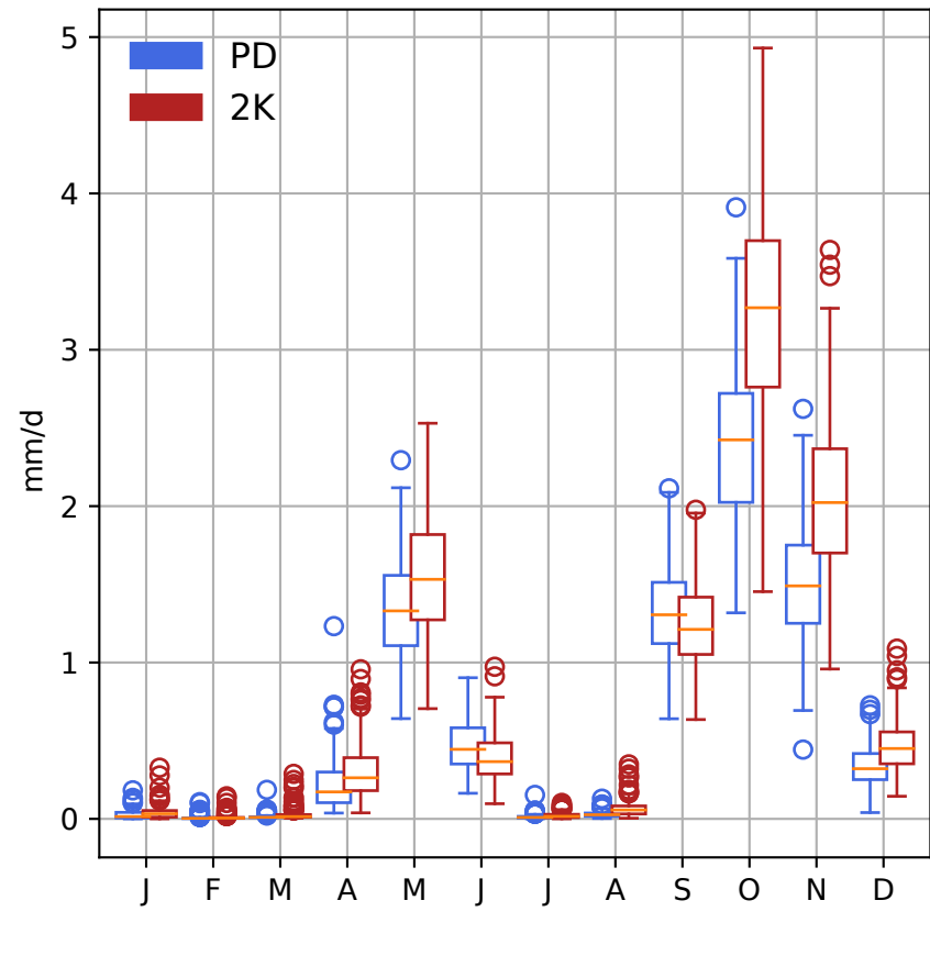
(c) Horn of Africa precipitation
