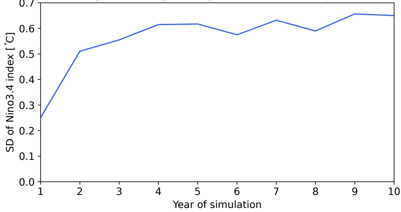
(b) Average variability among members of same parent
