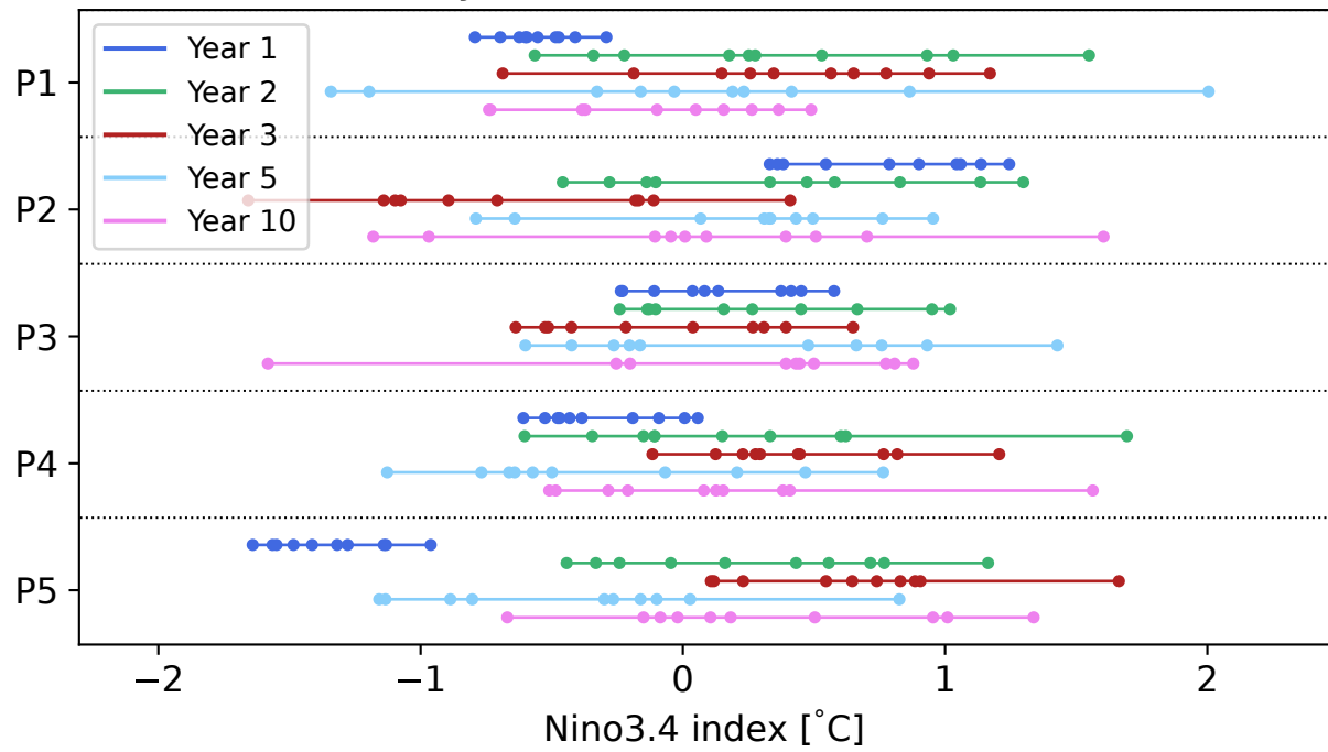
(a) ENSO variability in LENTIS-PD time slice
