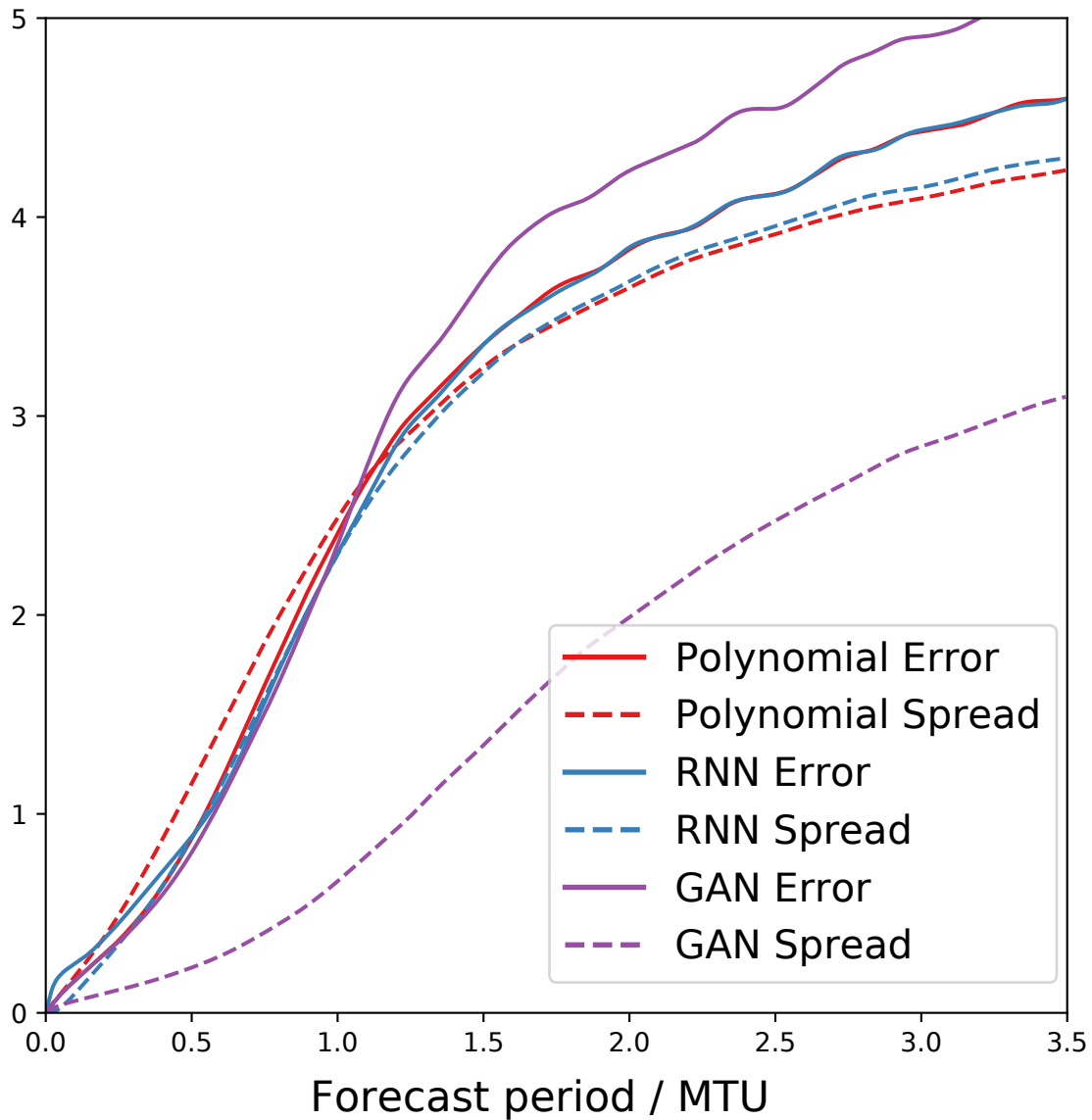
Spread-Error plot for F=20
