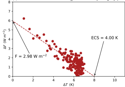
(c) v2LR_0101: 4xCO 2 Gregory plot
