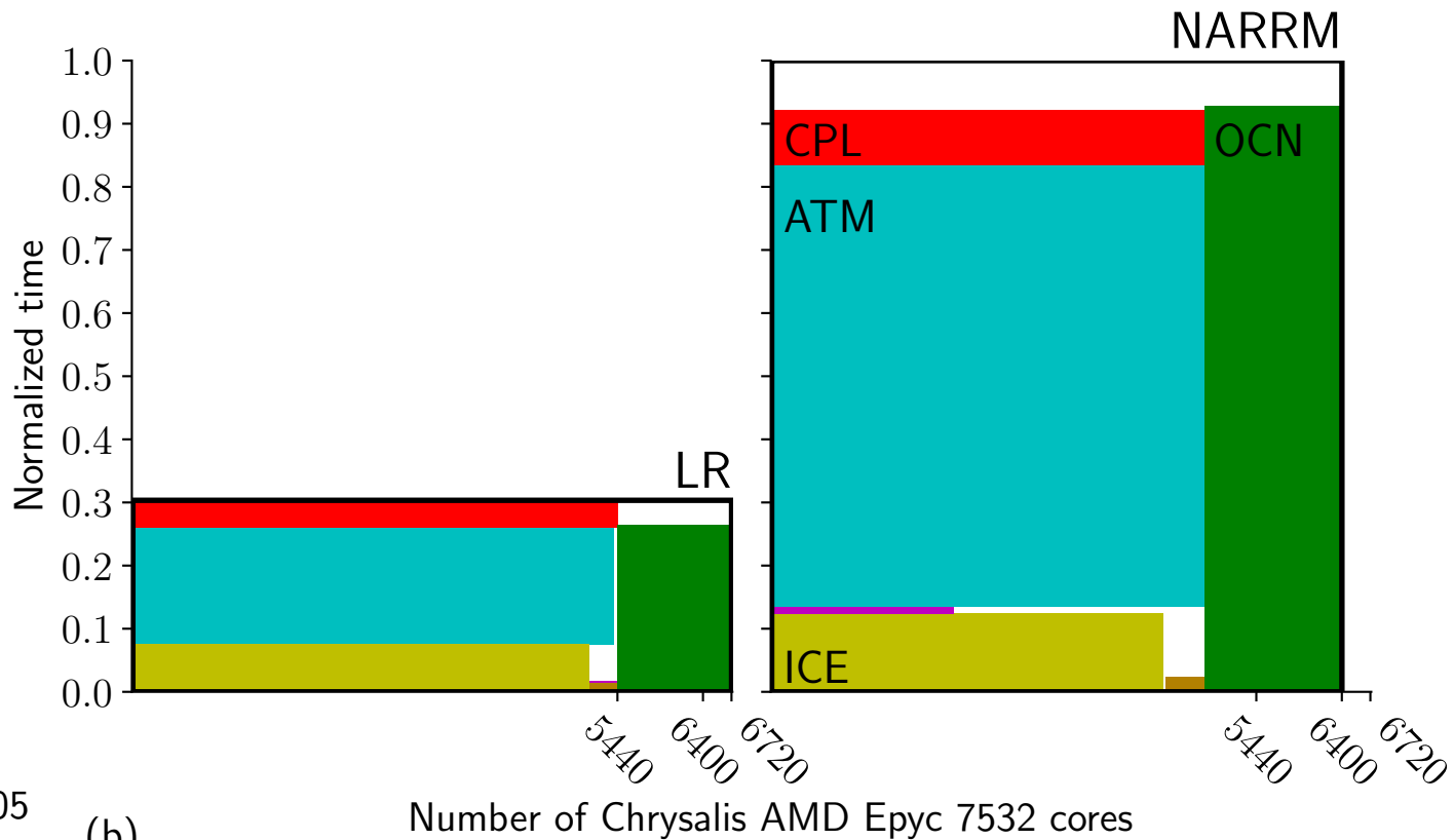
Performance of WCYCL20TR.ne30pg2_EC30to60E2r2 and WCYCL20TR.northamericax4v1pg2_WC14to60E2r3
