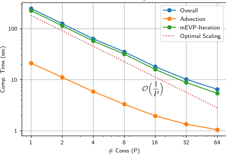
Parallel Scaling
