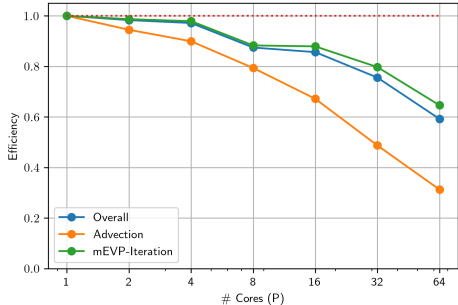
Parallel Efficiency
