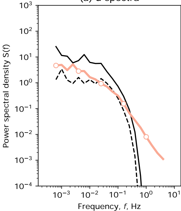
(a) u-spectra
