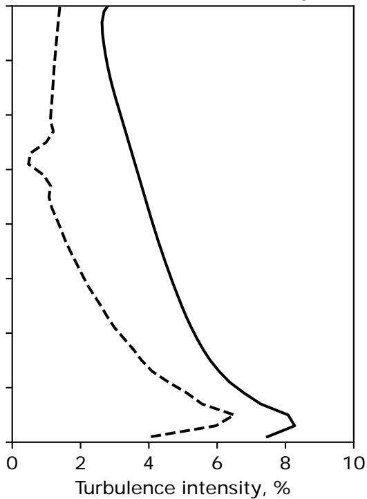
(b) Turbulence intensity
