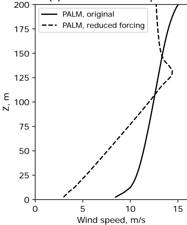
(a) Horizontal wind speed
