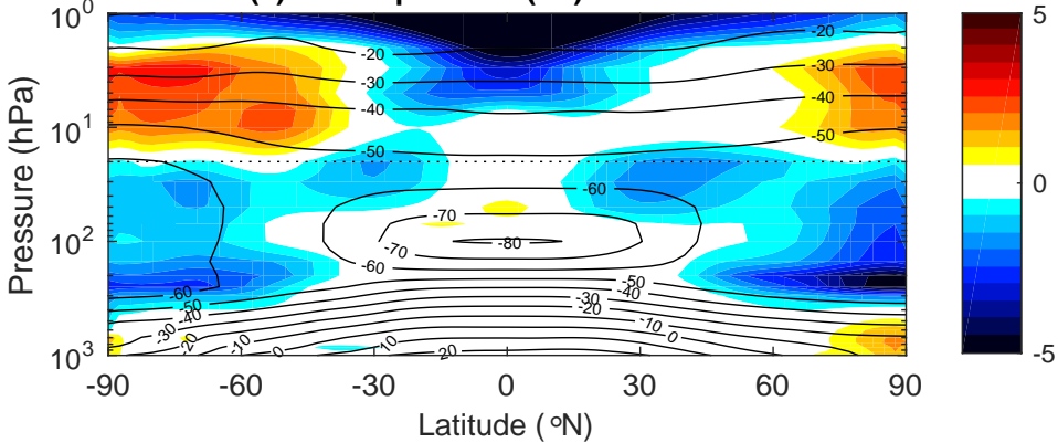
(b) \Delta Temperature ( ^{\circ}\text{C} ): Reduced SP
