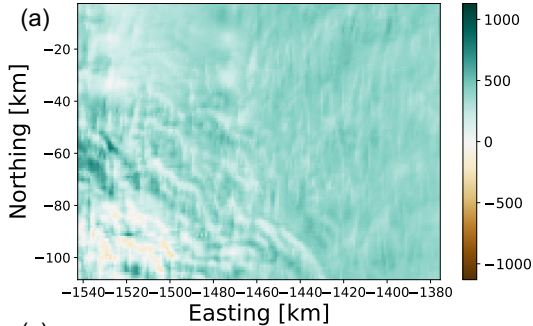
Liston 2015 Surface Mass Balance
