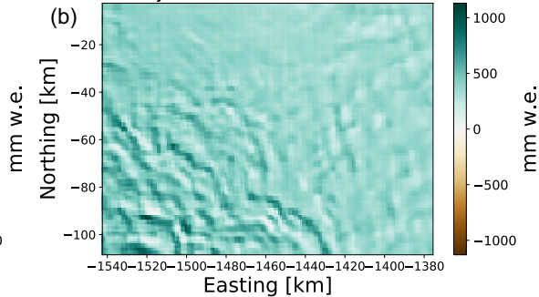
WindNinja 2015 Surface Mass Balance
