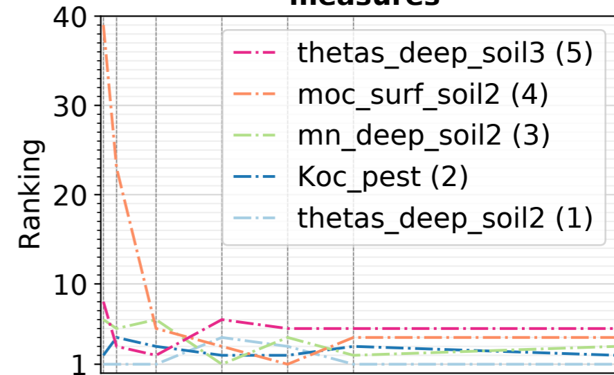
Feature importance measures
