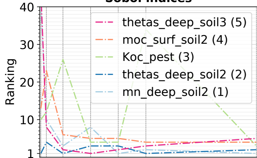
Sobol indices
