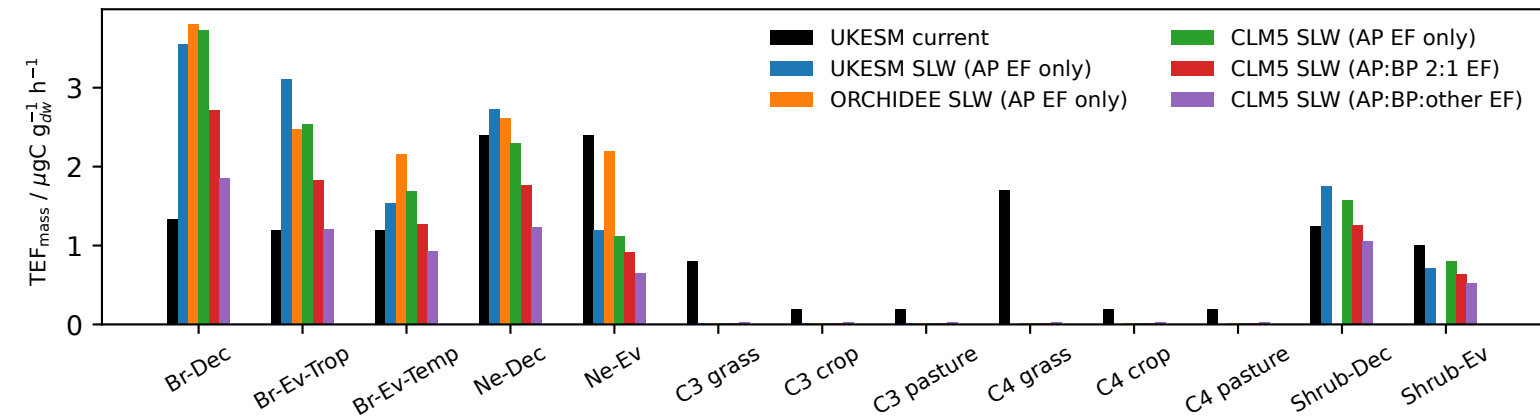
(b) TEF_{mass} on UKESM PFTs
