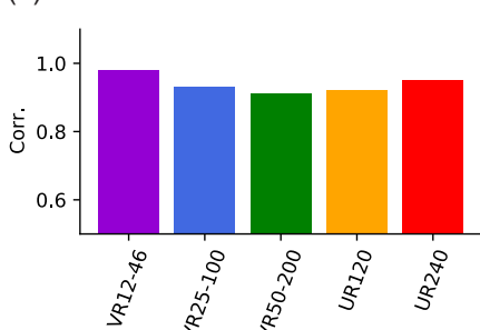
(e) Zonal wind at 200 hPa
