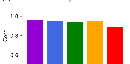
(c) Relative humidity at 850 hPa
