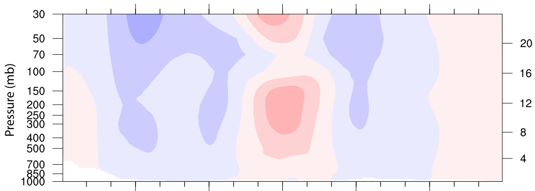
(e) [VR25-100] - [UR120]
