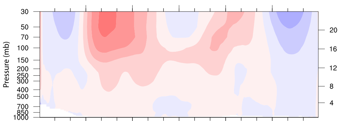
(c) [UR240] - [UR120]
