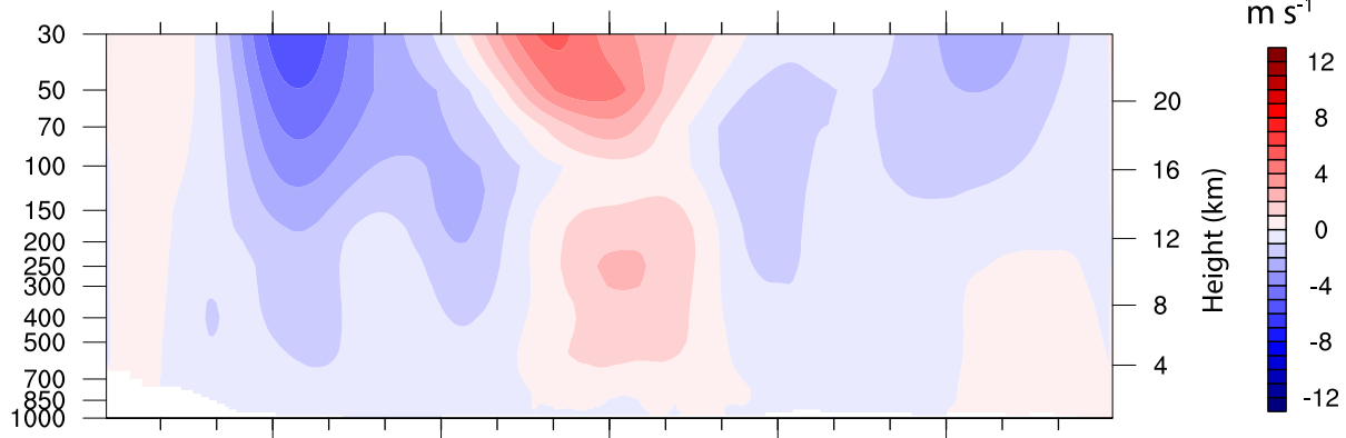
(f) [VR12-46] - [UR120]
