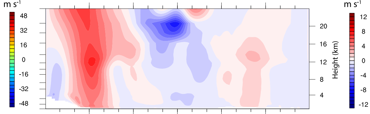
(b) [UR120] - [ERA-Interim]
