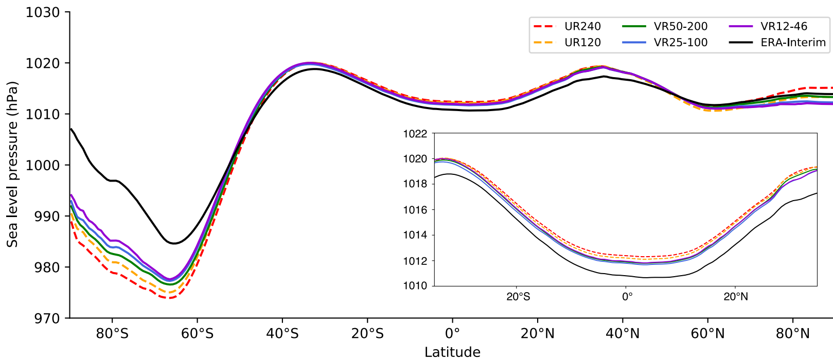
(b) Sea level pressure
