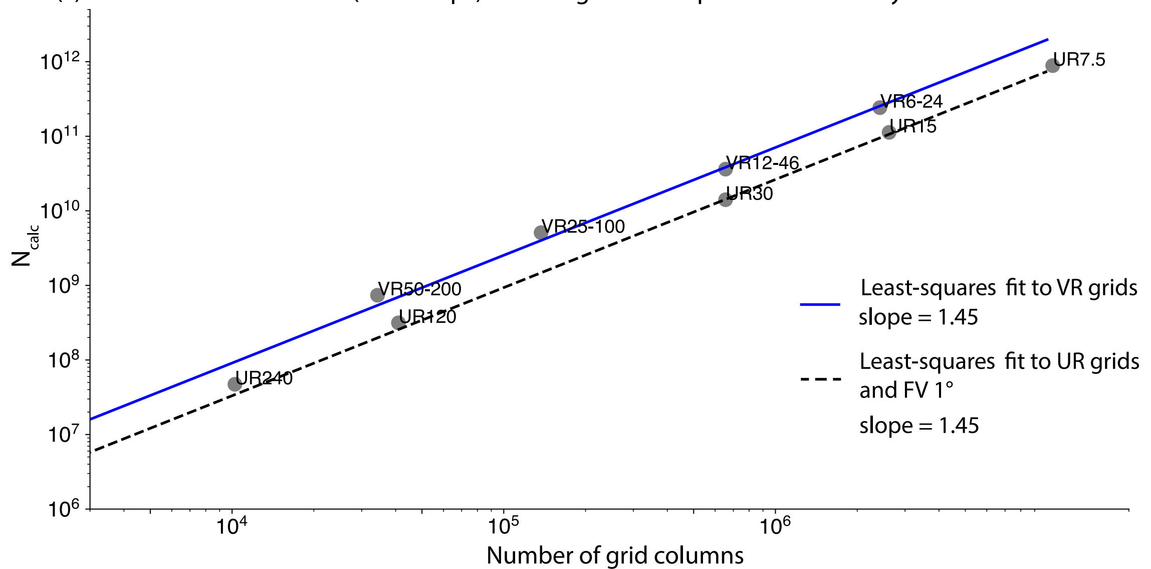
(c) Number of calculations (time steps) over all grid boxes per simulation day
