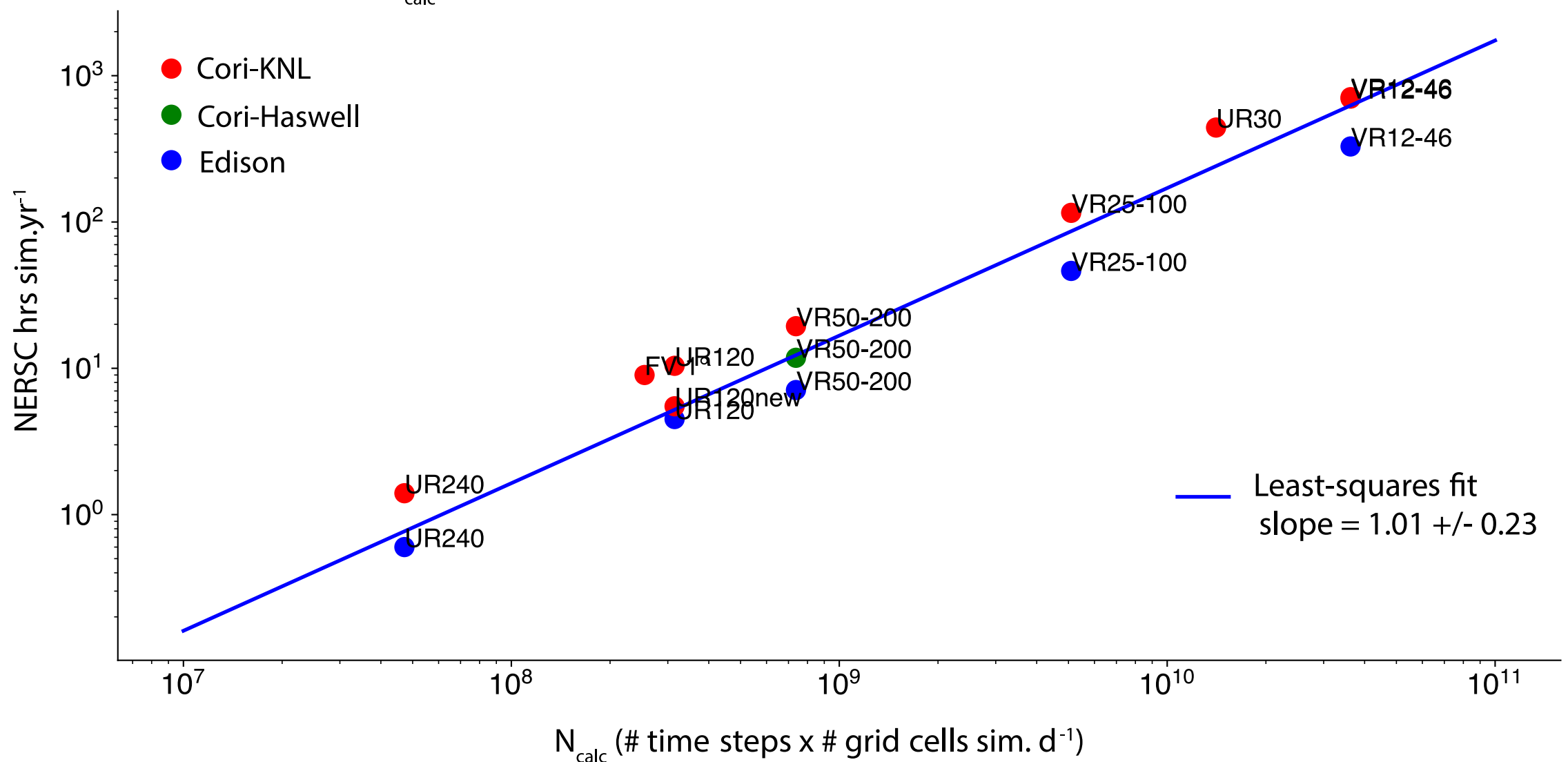
(b) Simulation cost vs. N_{\text{calc}}
