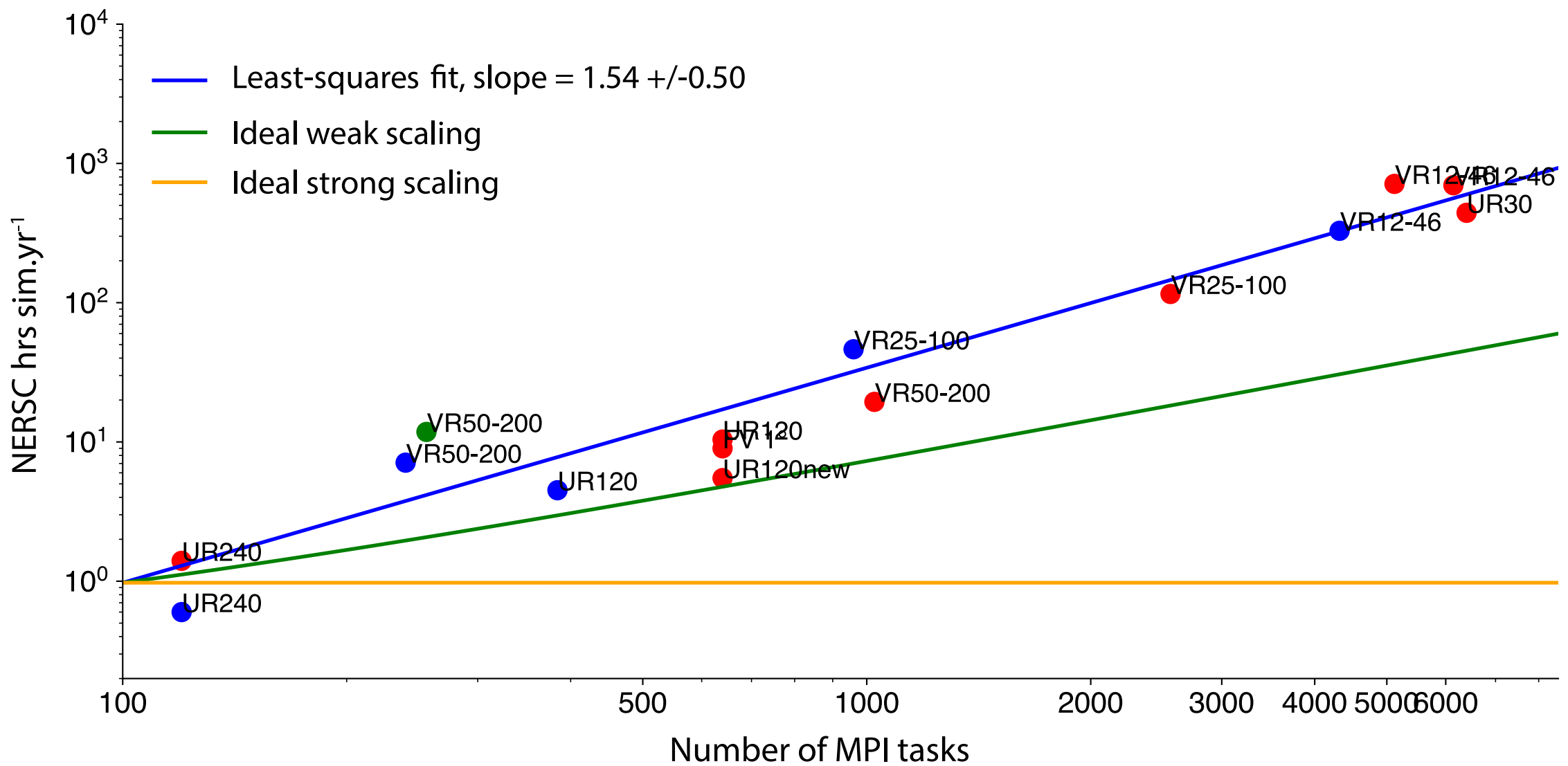
(a) Simulation cost vs. number of MPI tasks
