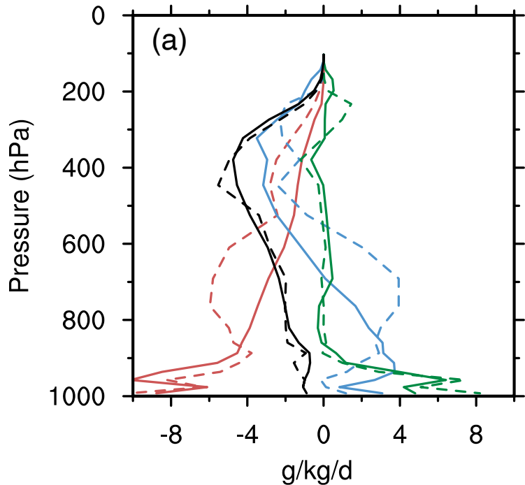
Convection-active period
