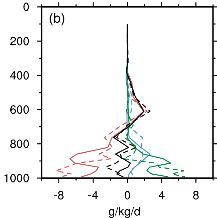
Convection-suppressed period
