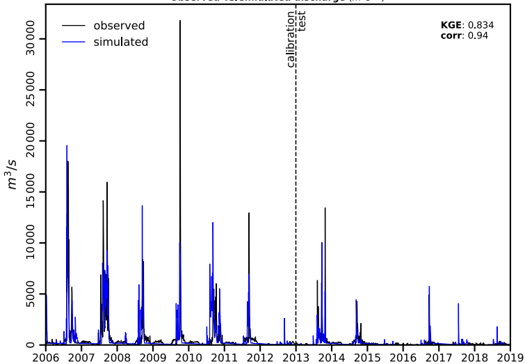
Observed vs. simulated discharge ( m^3s^{-1} )
