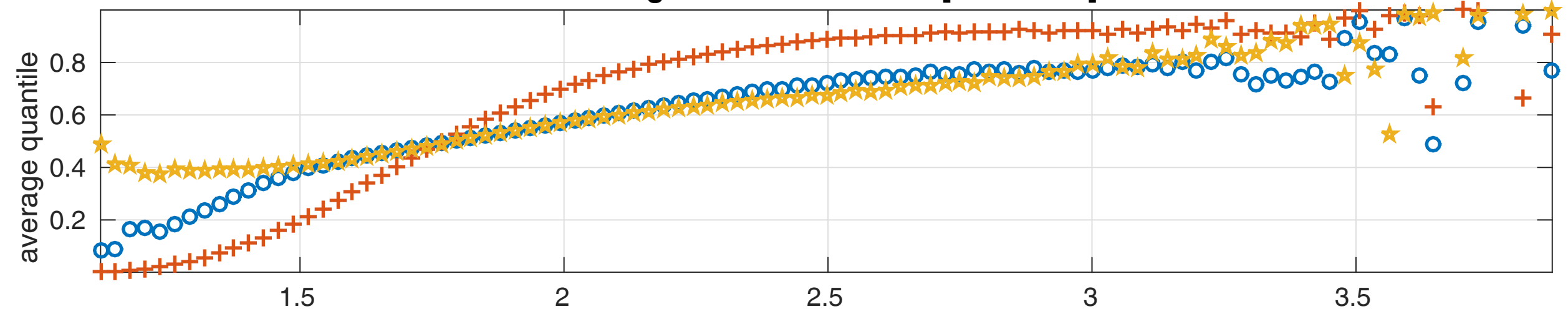
factors controlling sea level maximum [2020-2150]
