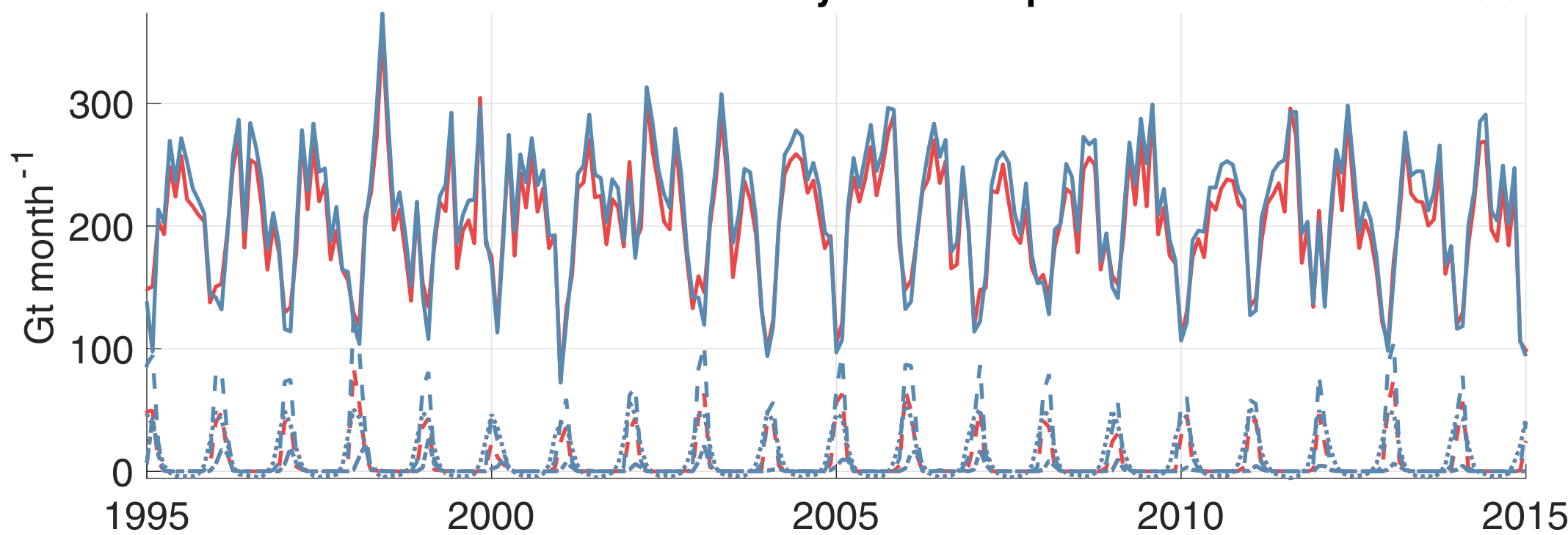
Antarctic: Monthly SMB components
