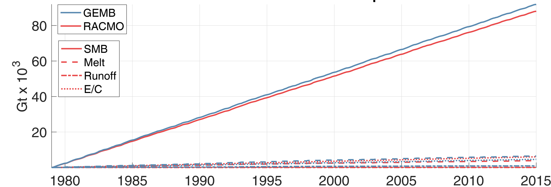
Antarctic: Cumulative SMB Components
