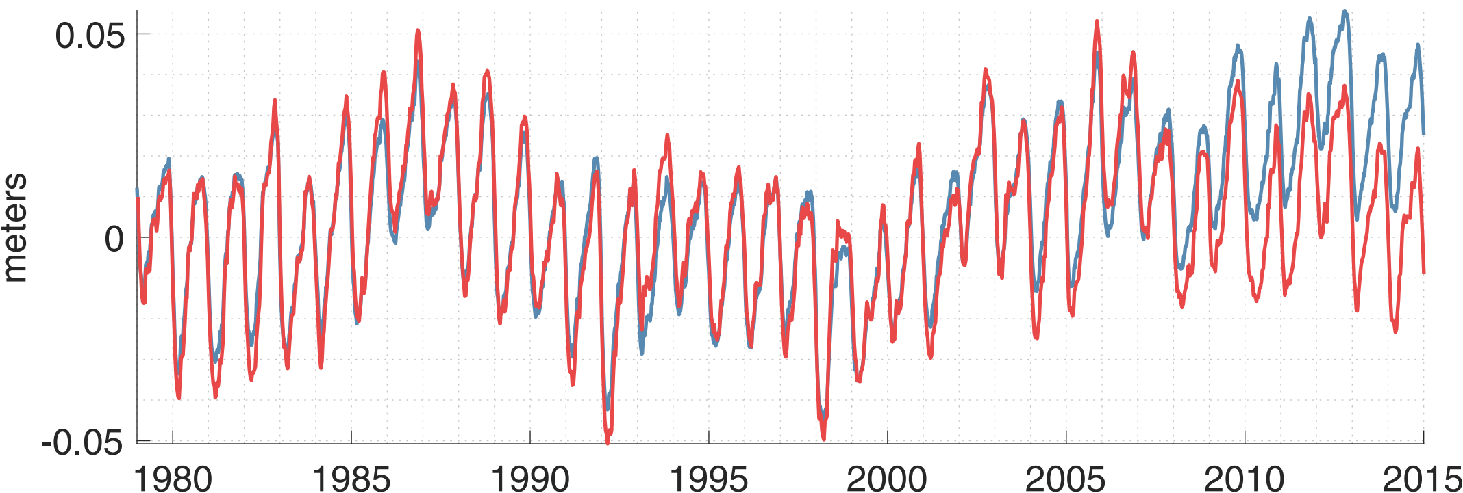
Antarctic: Firn Air Content
