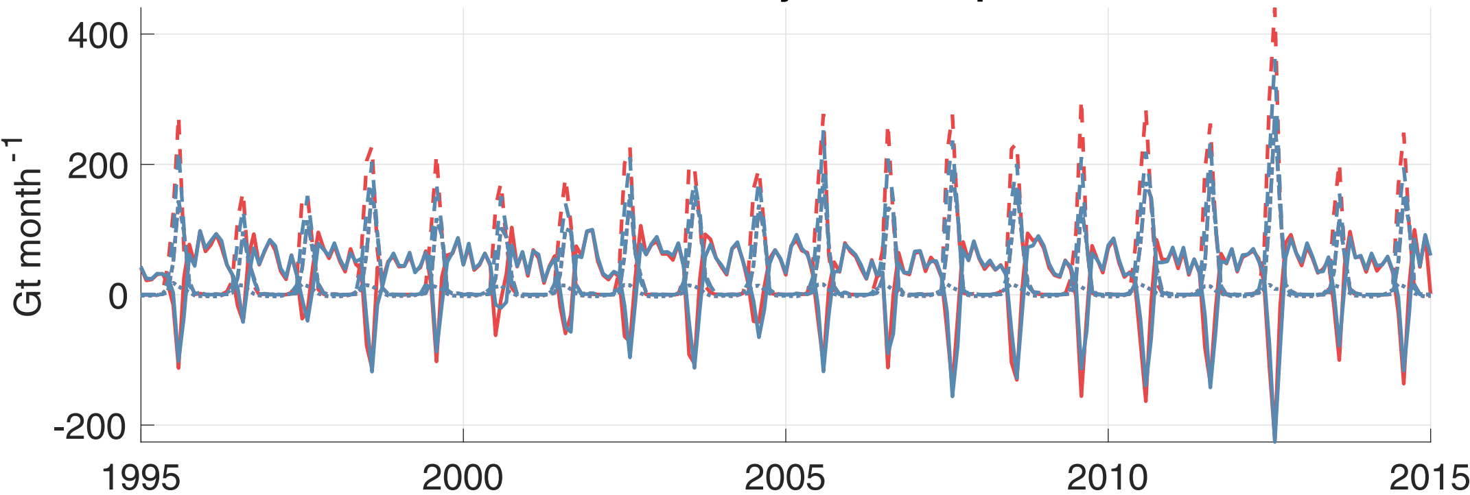
Greenland: Monthly SMB components
