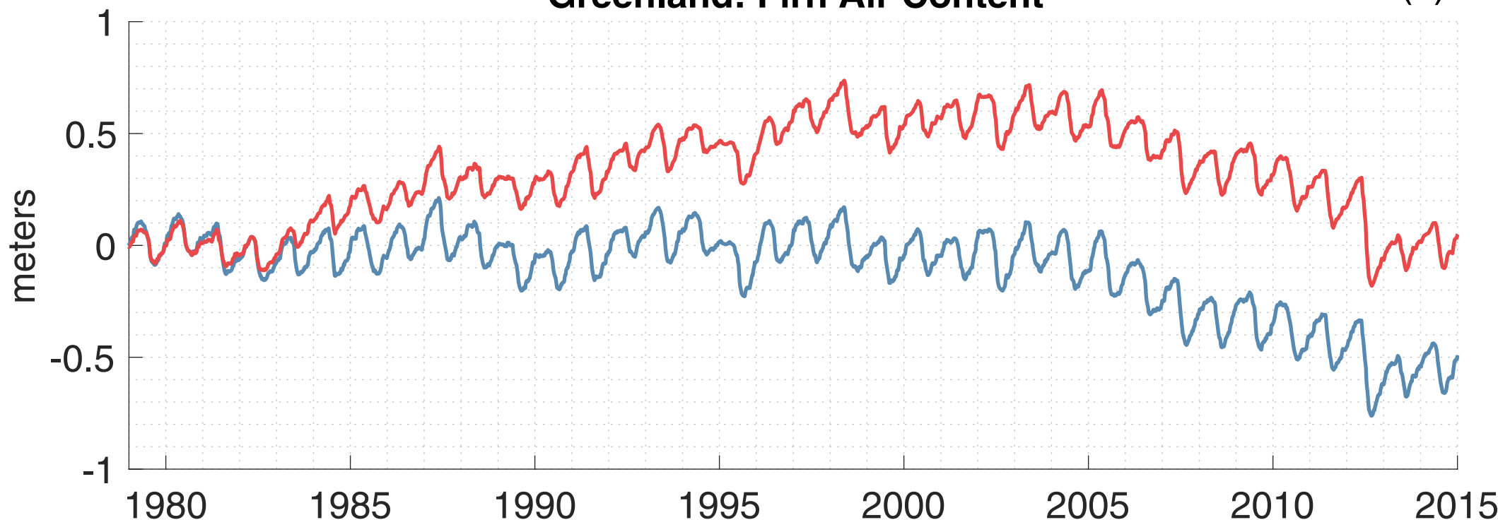
Greenland: Firn Air Content
