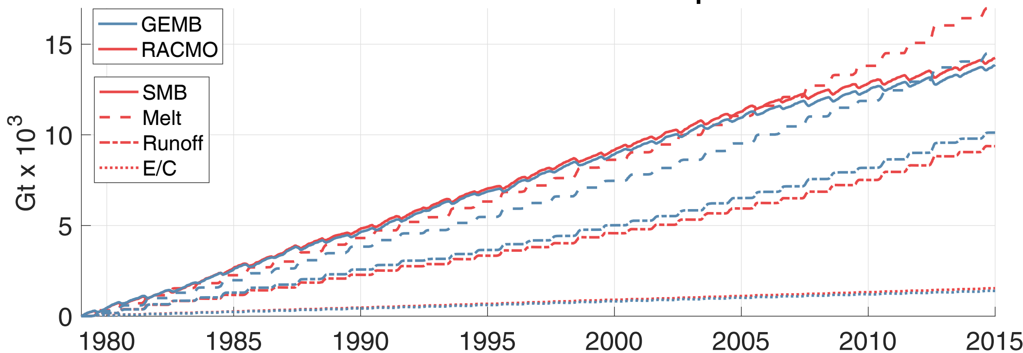
Greenland: Cumulative SMB Components
