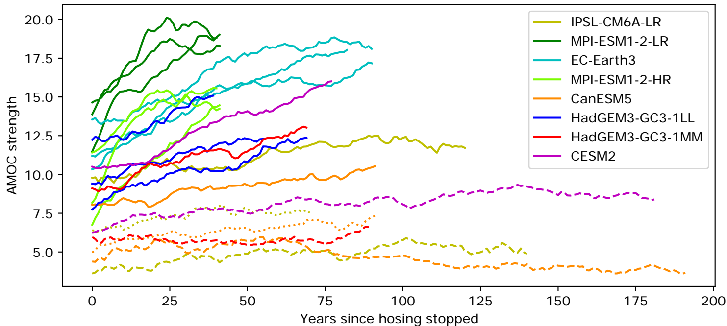
AMOC at 45°N
