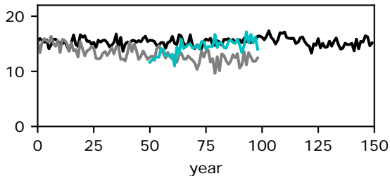
IPSL-CM6A-LR
