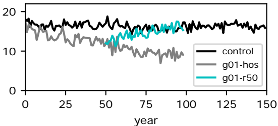
EC-Earth3
