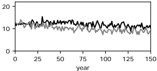
CanESM5
