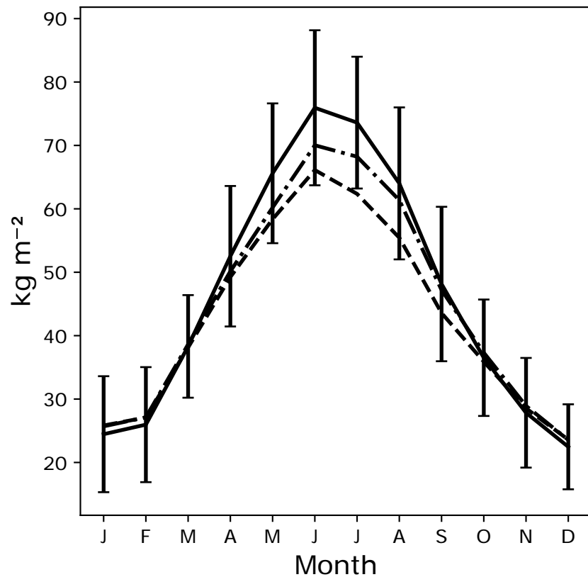
Change in Total Soil Moisture
