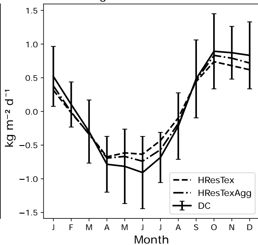
Change in Total Soil Moisture
