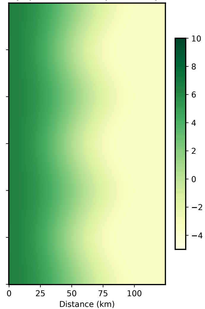
(c) U Wind ( \text{m s}^{-1} )
