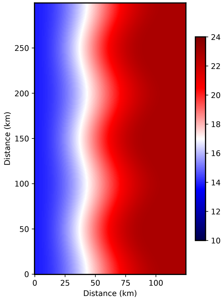
(a) T ( ^{\circ}\text{C} )
