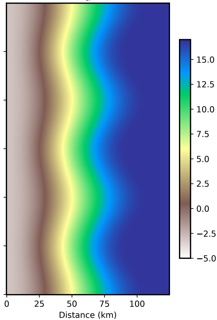
(b) T_d ( ^{\circ}\text{C} )
