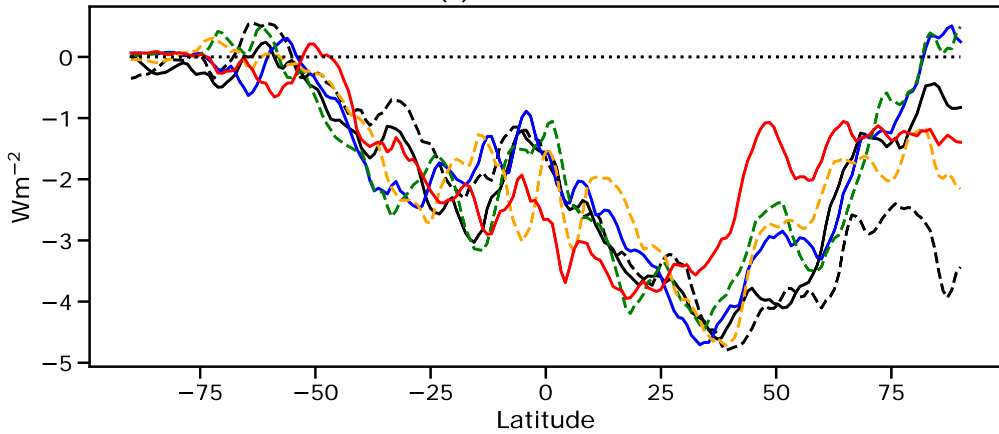
(c) \Delta TOM Residual PD-PI
