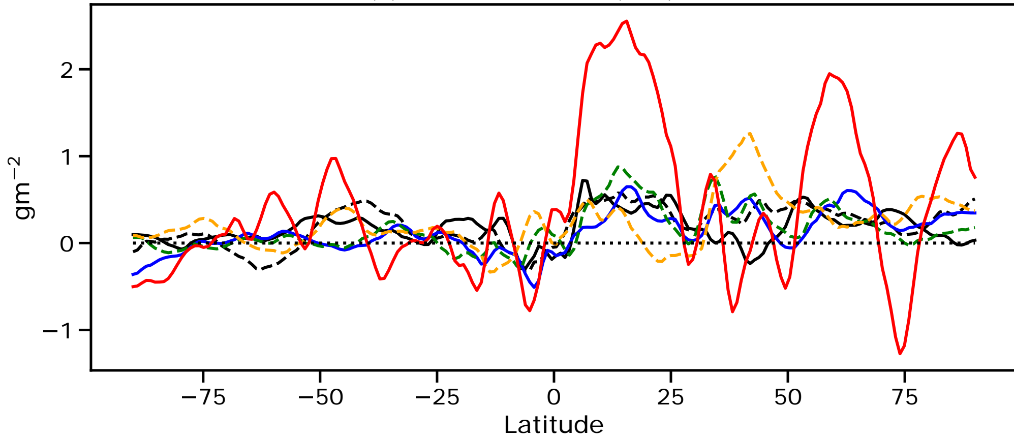
(e) \Delta Ice Water Path (IWP) PD-PI
