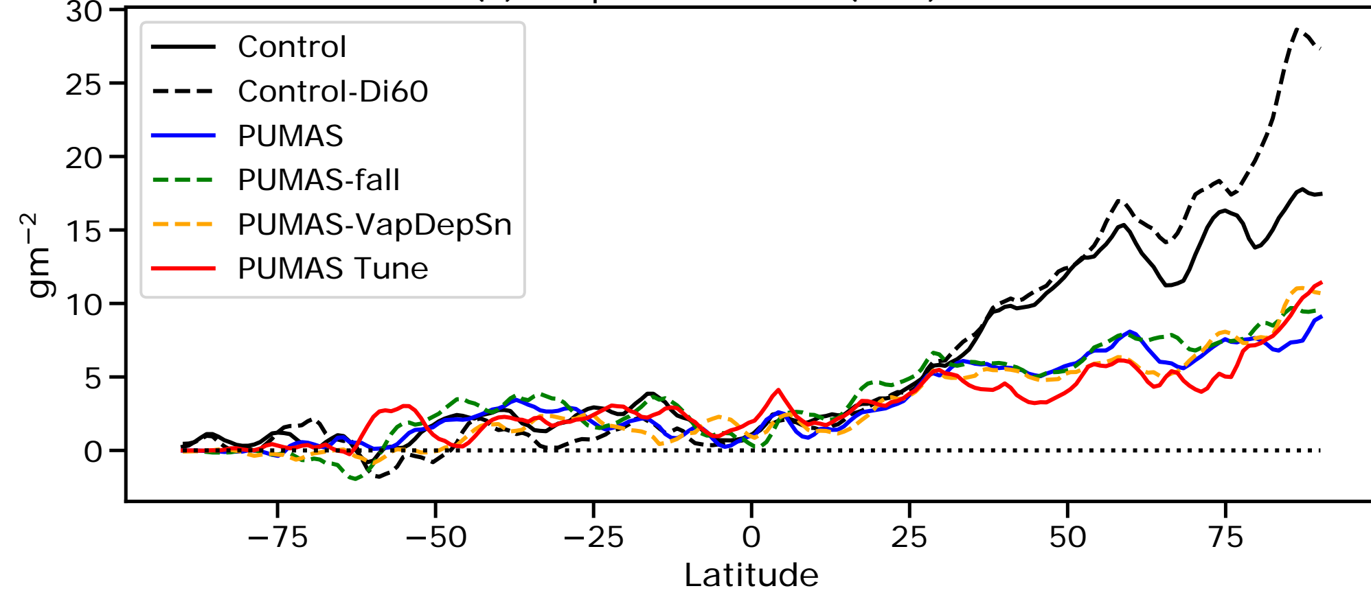
(f) \Delta Column Cld Drop Number PD-PI
