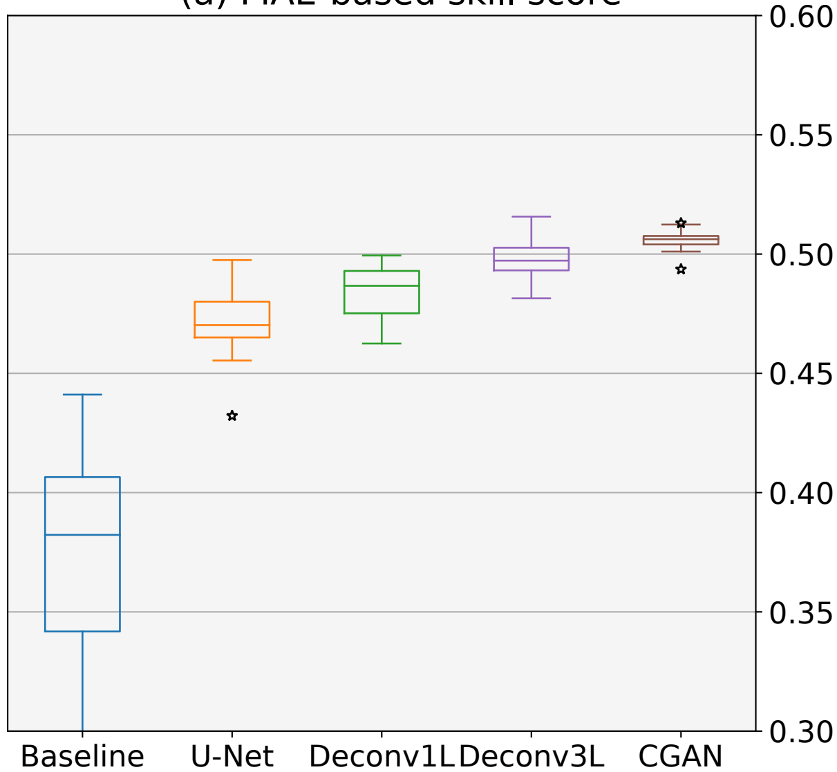
(a) MAE-based skill score
