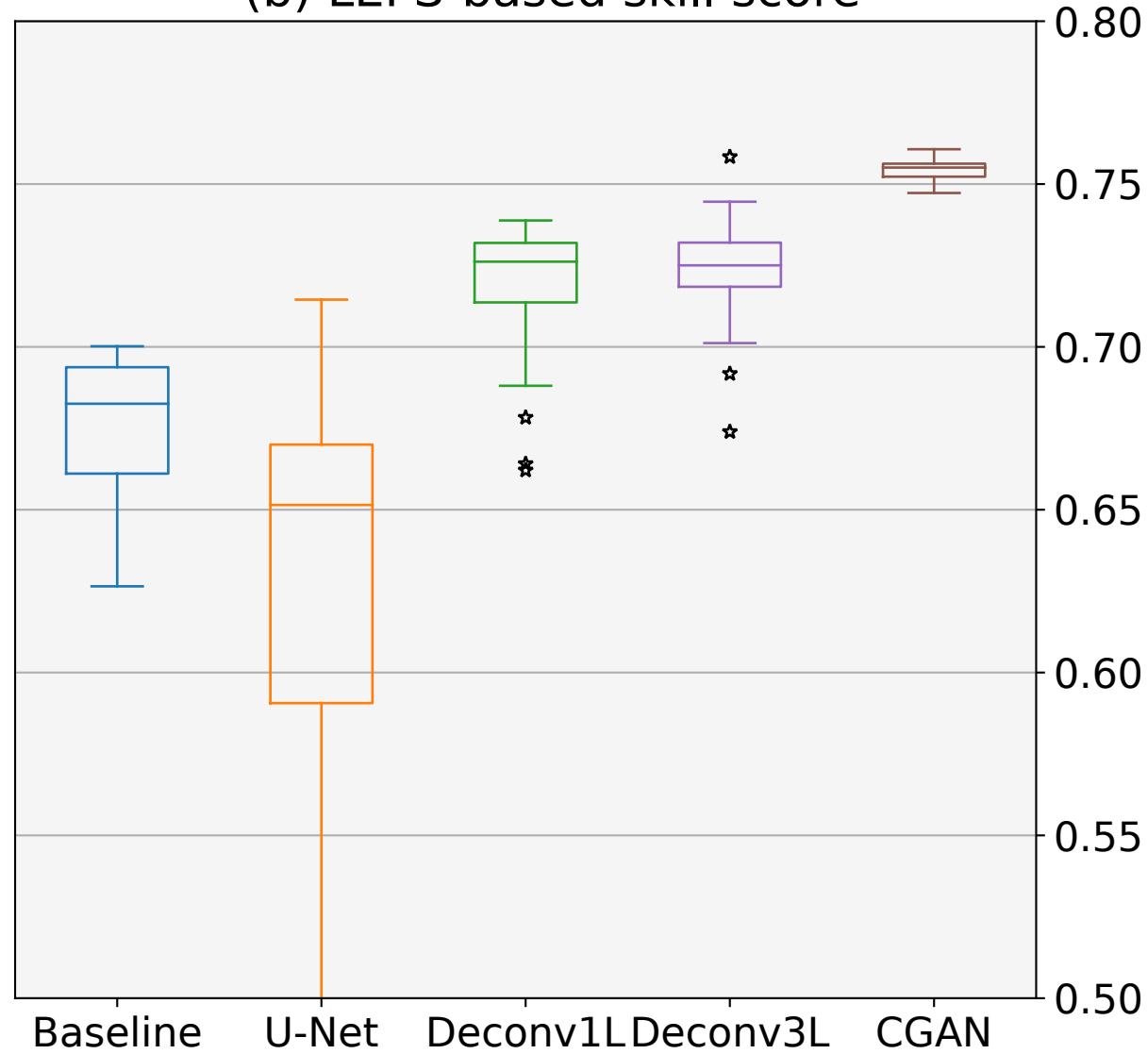
(b) LEPS-based skill score
