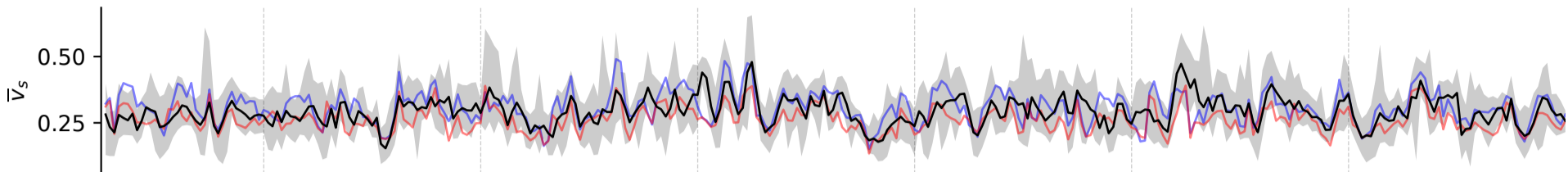
North Madagascar Current
