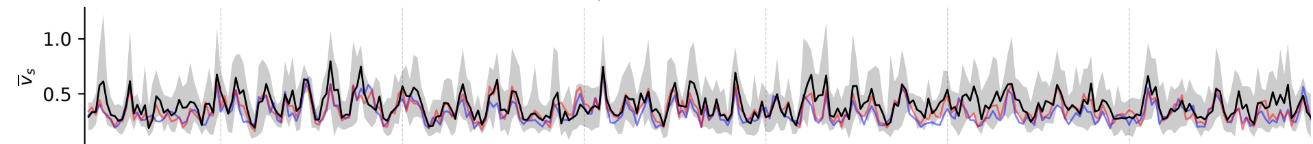
South Equatorial Countercurrent (East)
