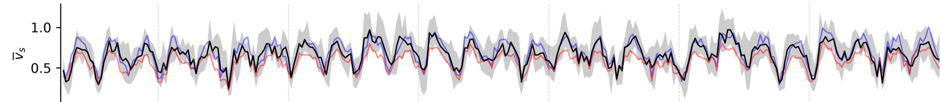
East Madagascar Current
