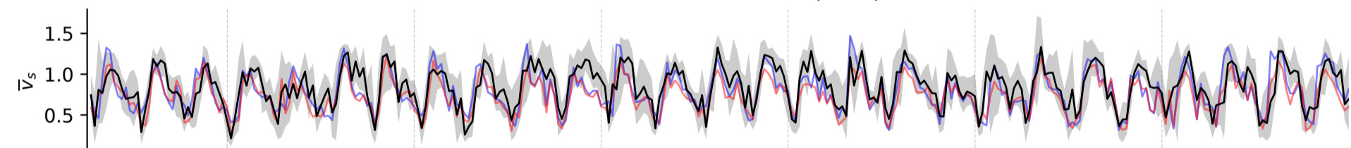
East Africa Coastal Current (South)
