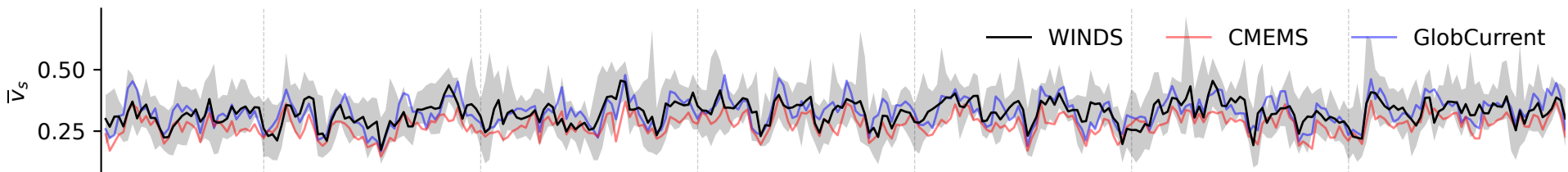
South Equatorial Current (East)
