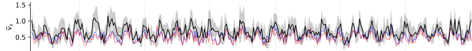
SW Mozambique Channel
