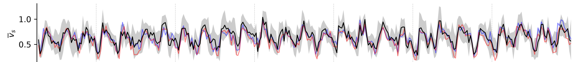
South Equatorial Countercurrent (West)
