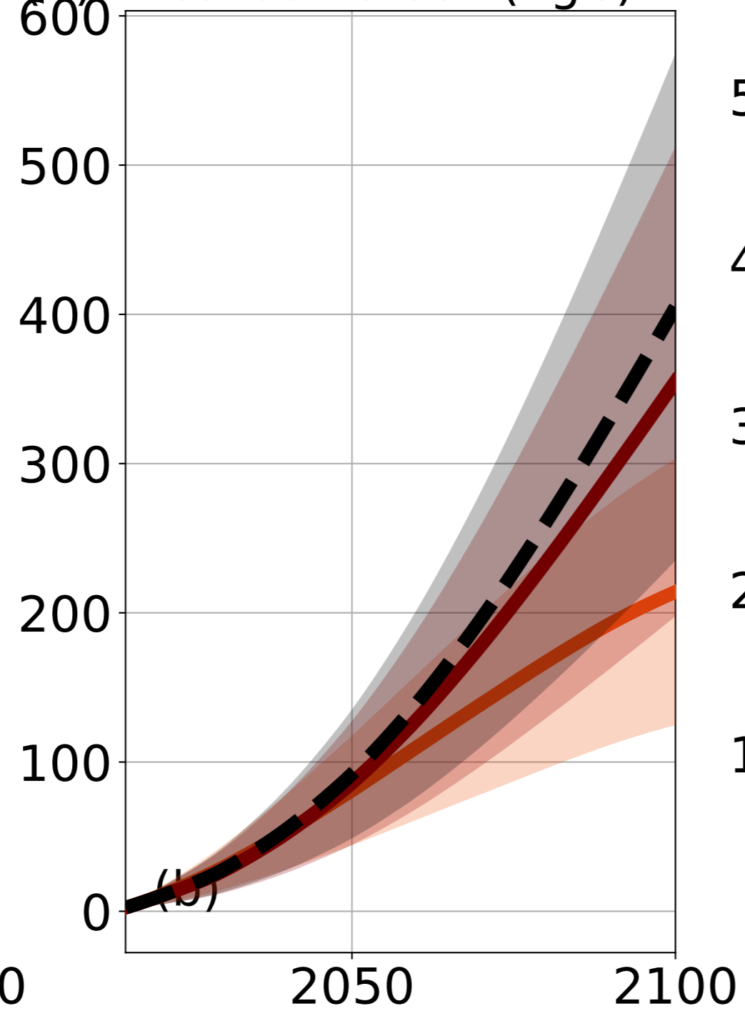
Change in land carbon stock (PgC)
