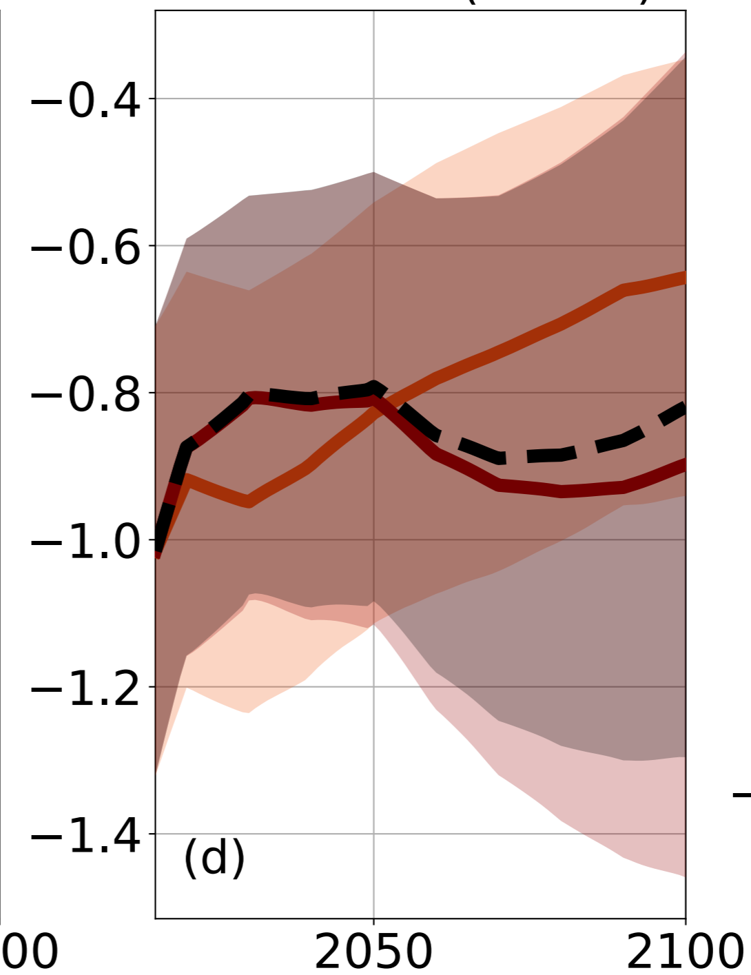
Radiative forcing of aerosols ( \text{W}\cdot\text{m}^{-2} )
