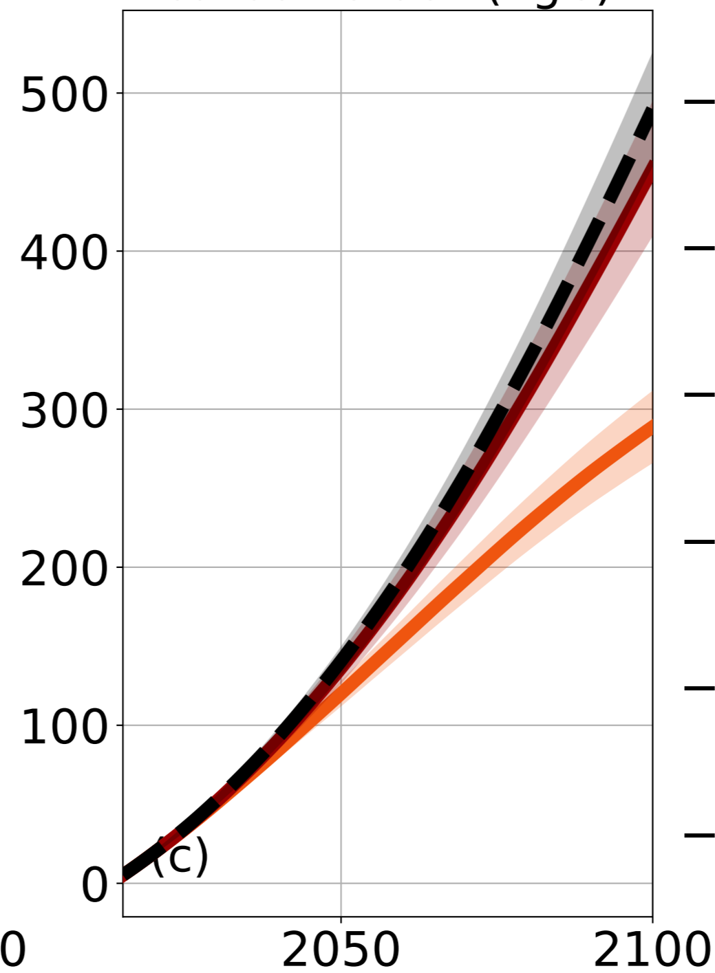
Change in oceanic carbon stock (PgC)
