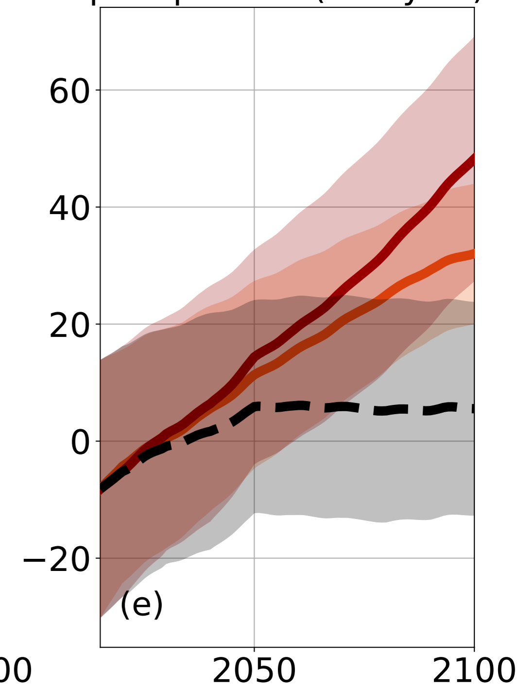
Change in global precipitation ( \text{mm}\cdot\text{yr}^{-1} )
