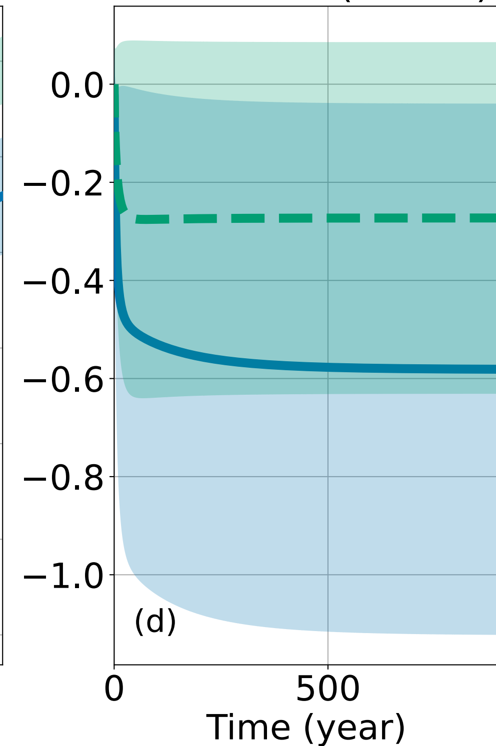
Radiative forcing of aerosols ( \text{W}\cdot\text{m}^{-2} )
