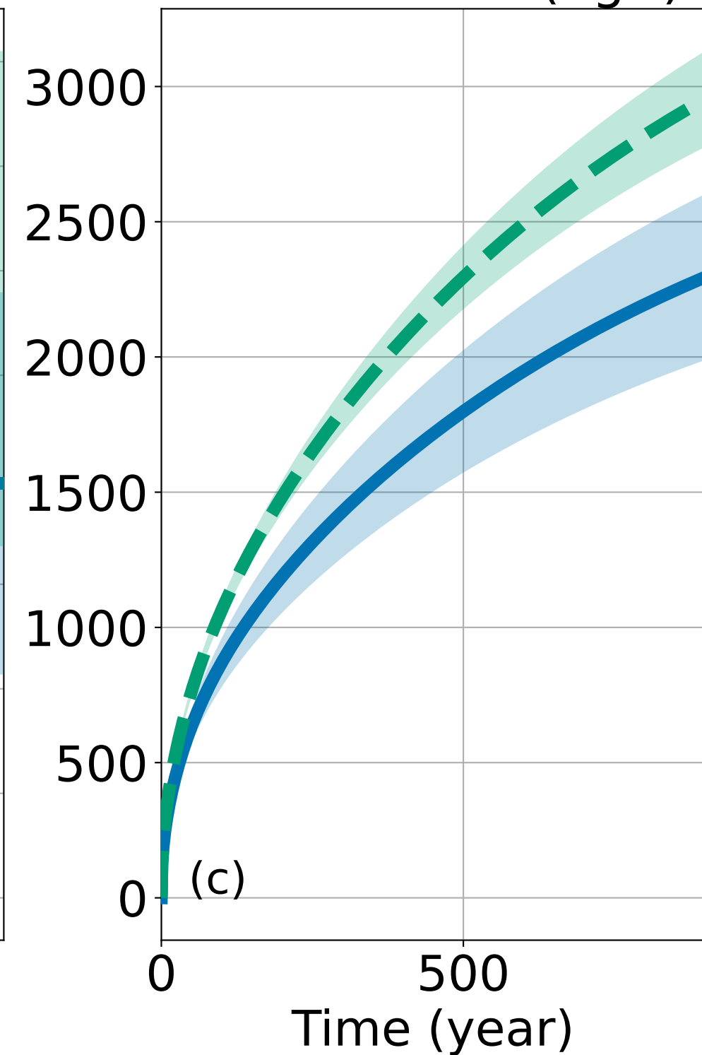
Change in oceanic carbon stock (PgC)
