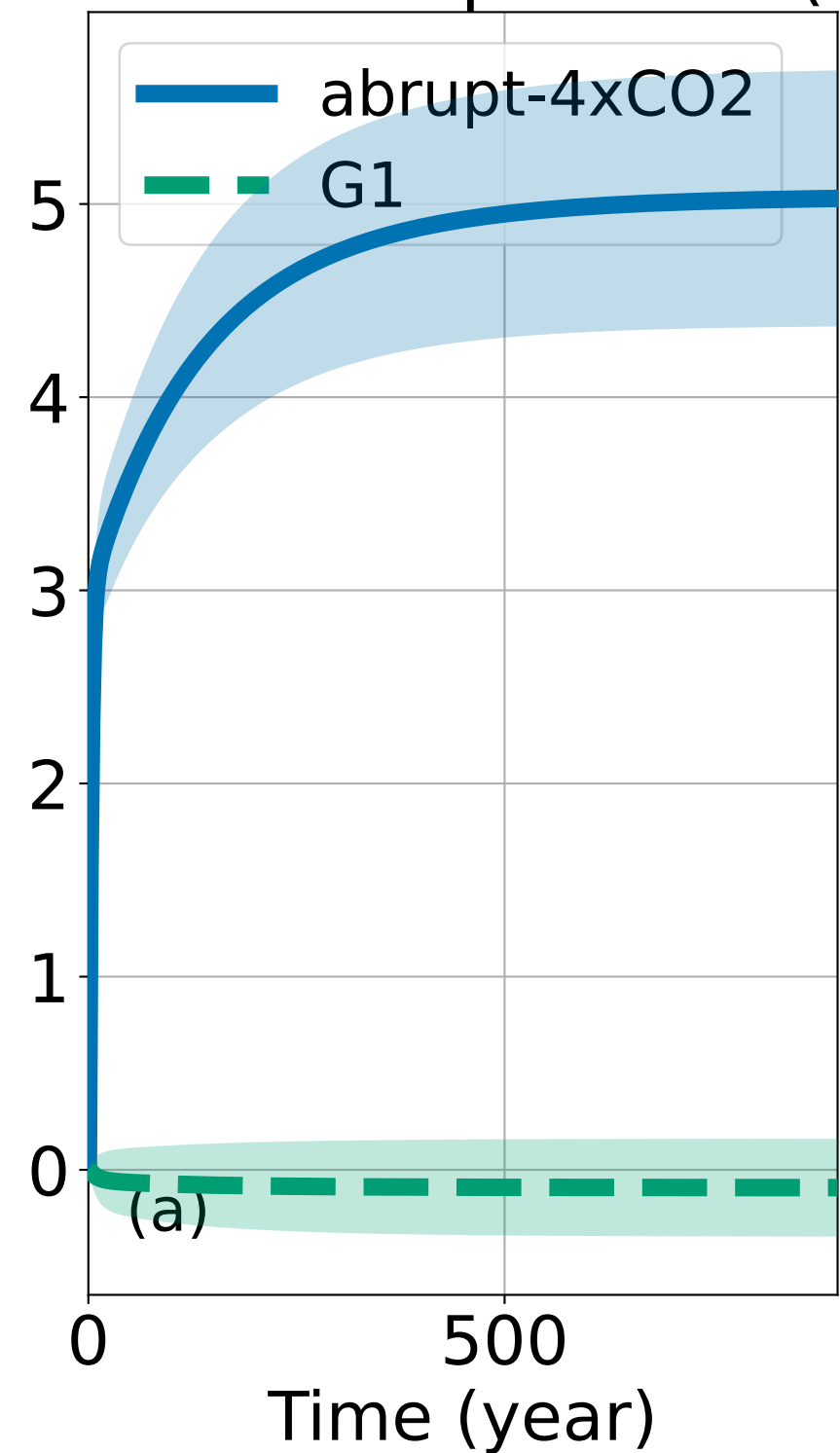
Change in global mean surface temperature (K)
