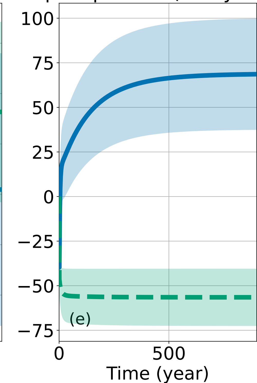
Change in global precipitation ( \text{mm}\cdot\text{yr}^{-1} )
