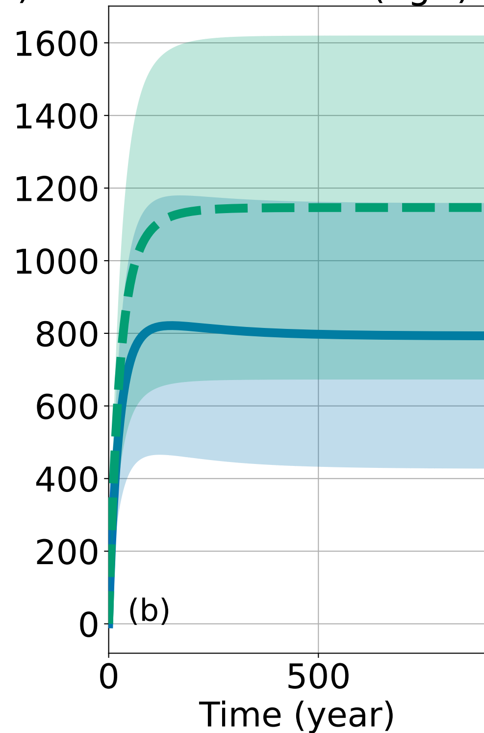
Change in land carbon stock (PgC)
