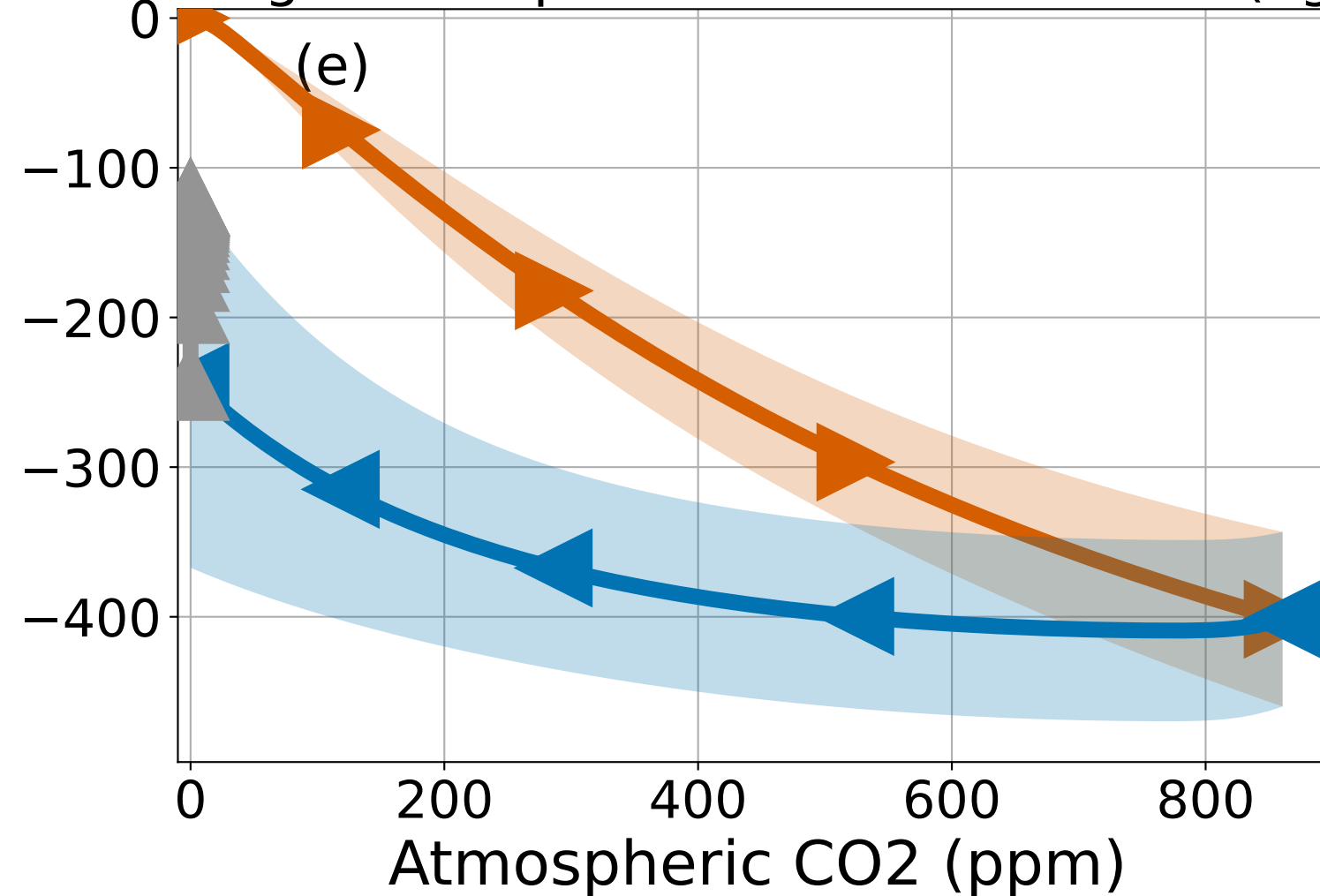
Change in the permafrost carbon stock (PgC)
