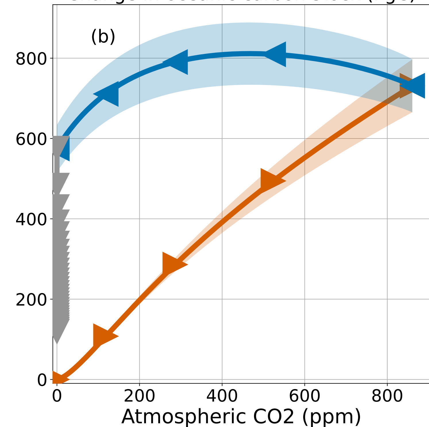
Change in oceanic carbon stock (PgC)
