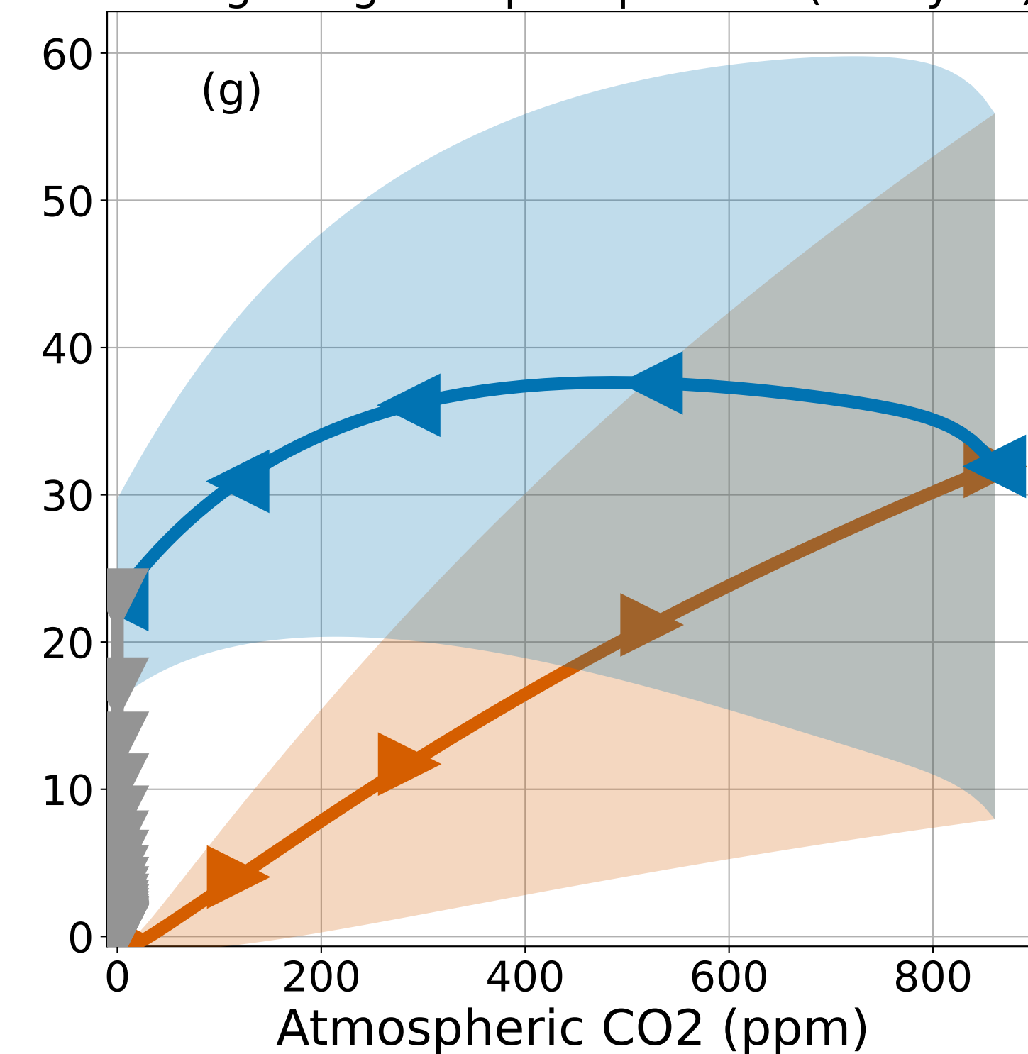
Change in global precipitation (mm.yr -1 )
