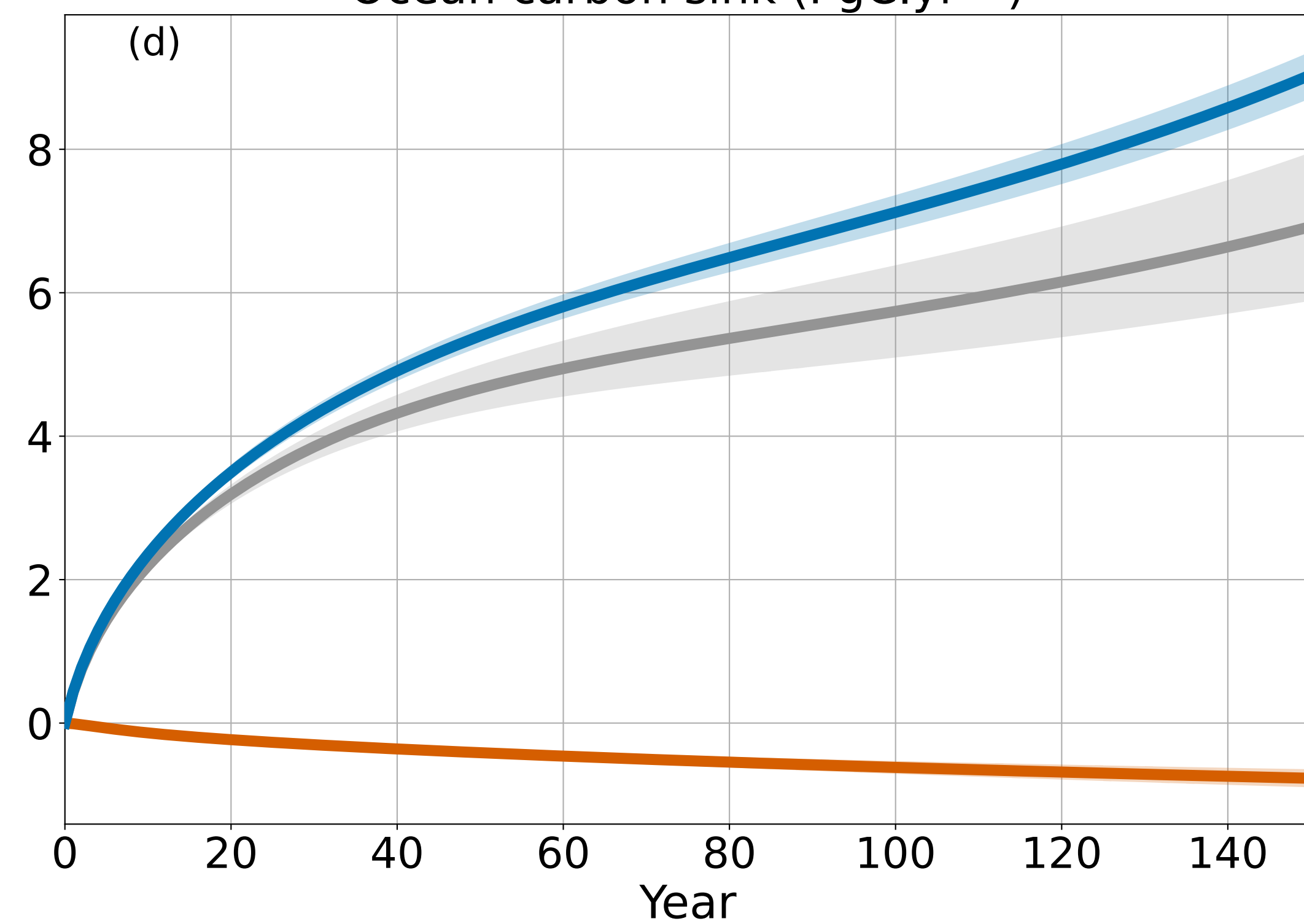
Ocean carbon sink (PgC.yr -1 )
