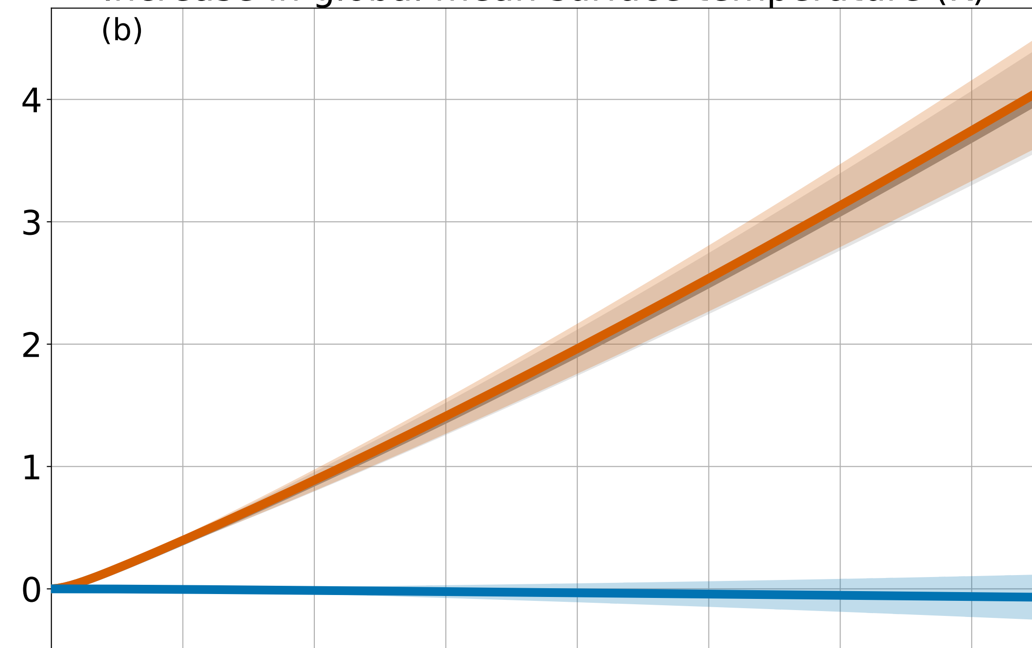
Increase in global mean surface temperature (K)
