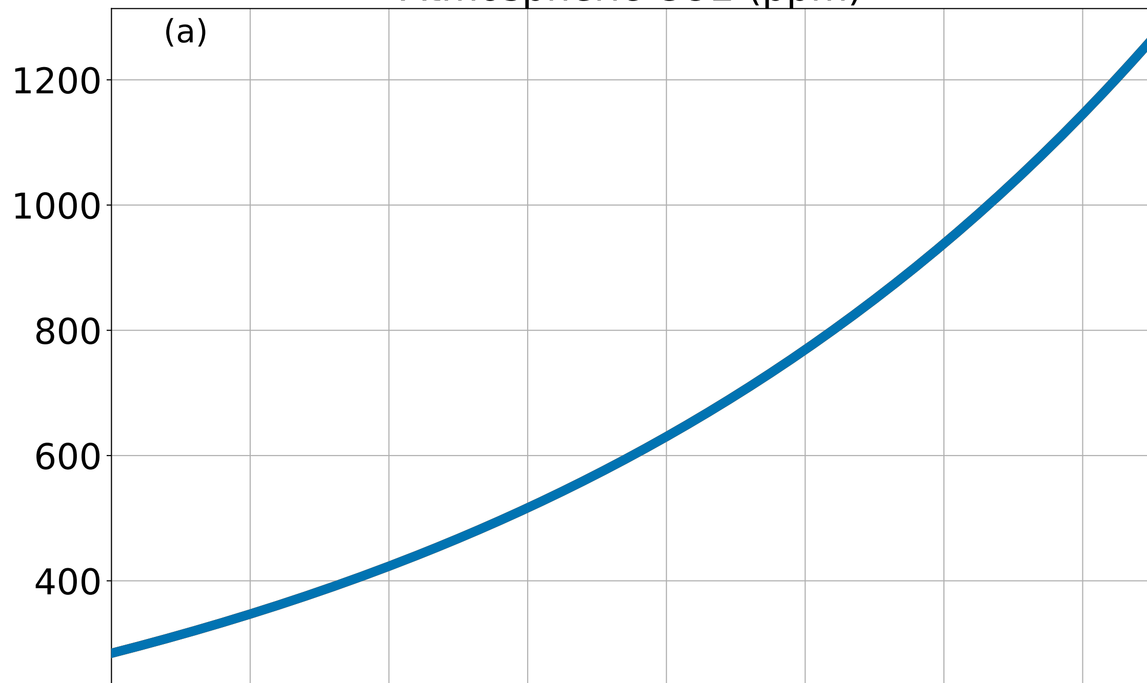
Atmospheric CO2 (ppm)
