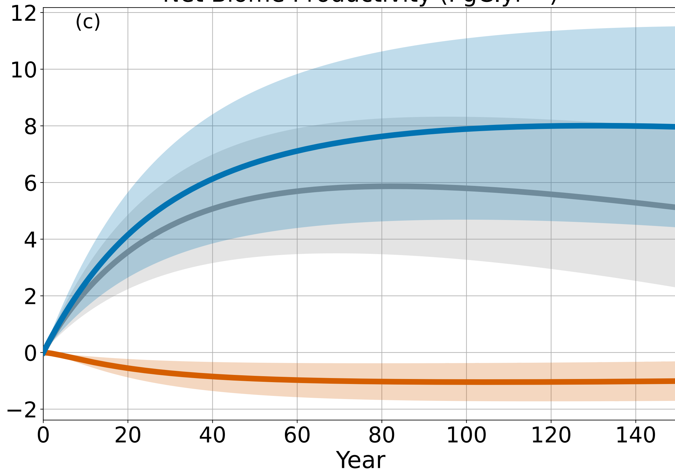
Net Biome Productivity (PgC.yr -1 )
